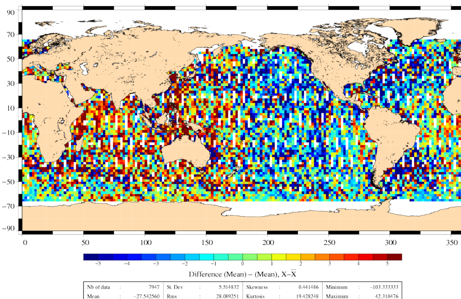
Differences of SLA before orbit error correction J2 – EN (17/02/2010 to 26/02/2010)
