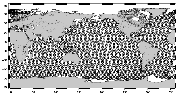
ENVISAT 10-day coverage for Jason-2 cycle 61
