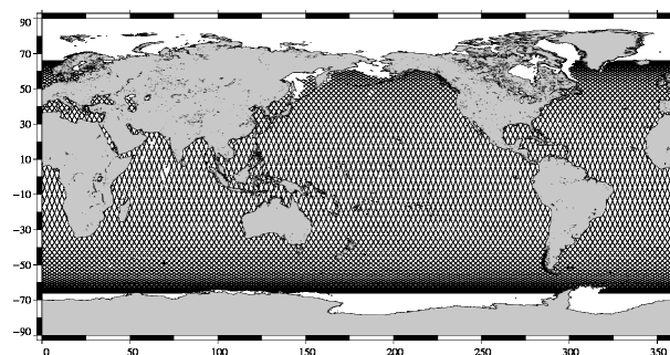
JASON 2 10-day coverage for Jason-2 cycle 61
