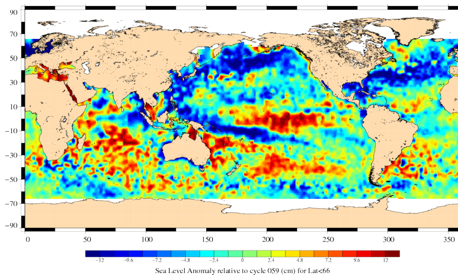
Variability relative to MSS (cm) Cycle 060 EN (17/02/2010 to 26/02/2010)
