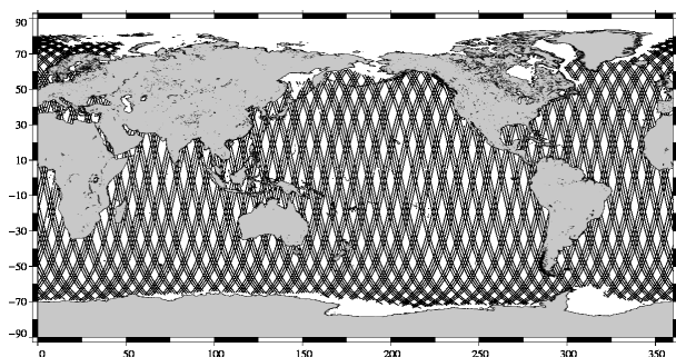
ENVISAT 10-day coverage for Jason-2 cycle 64
