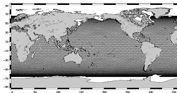
JASON 2 10-day coverage for Jason-2 cycle 64
