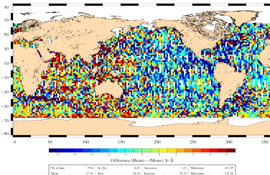
Differences of SLA before orbit error correction J2 – EN (18/03/2010 to 28/03/2010)
