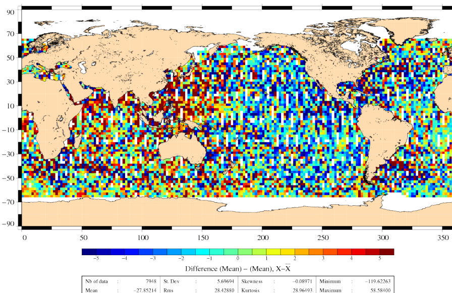
Differences of SLA before orbit error correction J2 – EN (28/03/2010 to 07/04/2010)
