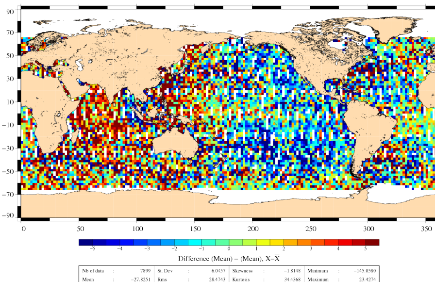
Differences of SLA before orbit error correction J2 – EN (07/05/2010 to 17/05/2010)
