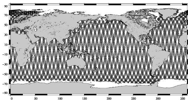
ENVISAT 10-day coverage for Jason-2 cycle 69
