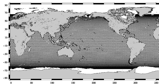
JASON 2 10-day coverage for Jason-2 cycle 69
