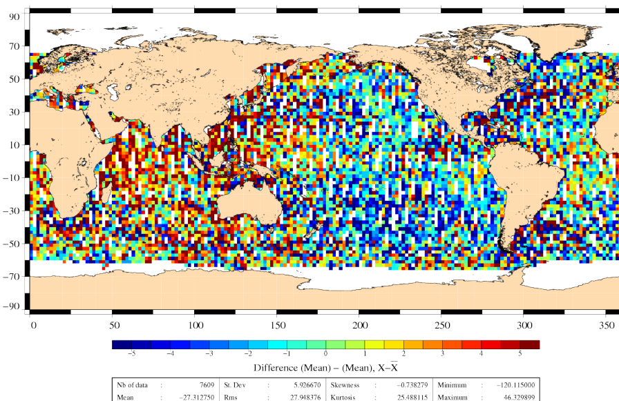
Differences of SLA before orbit error correction J2 – EN (16/06/2010 to 25/06/2010)
