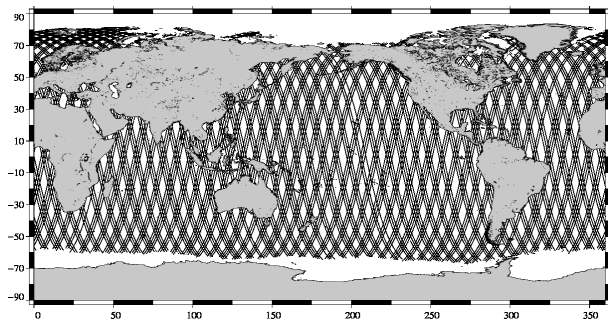
ENVISAT 10-day coverage for Jason-2 cycle 74
