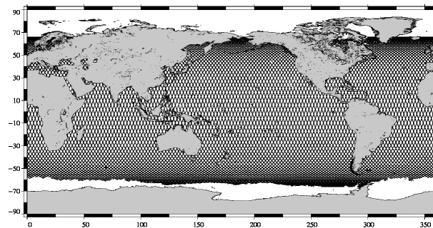
JASON 2 10-day coverage for Jason-2 cycle 74
