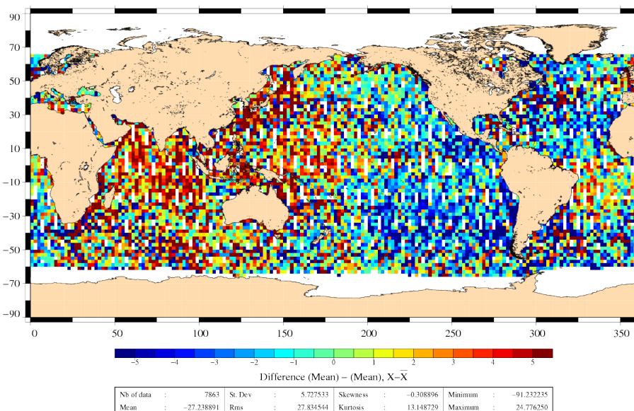
Differences of SLA before orbit error correction J2 – EN (25/06/2010 to 05/07/2010)
