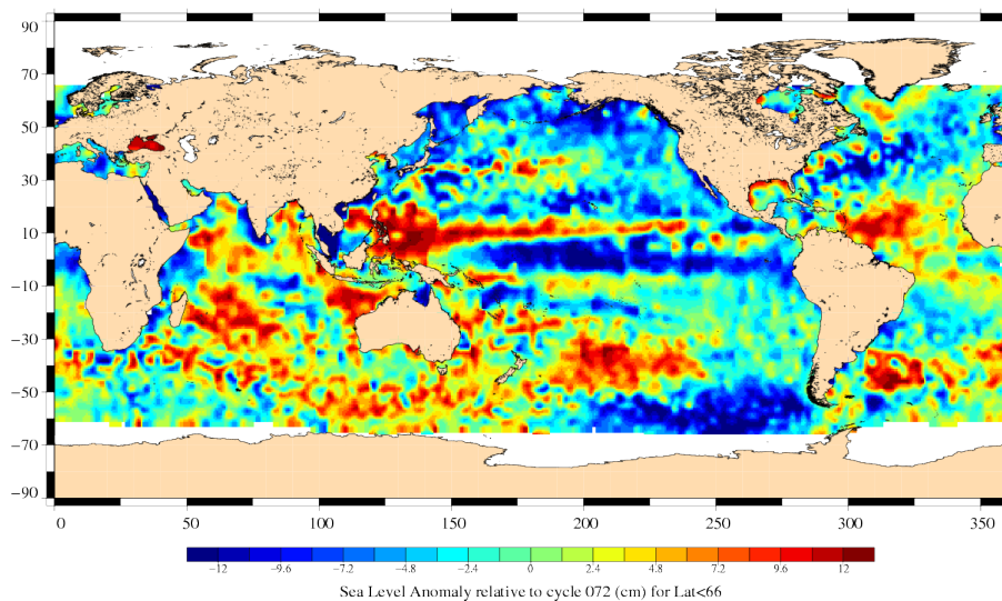
Variability relative to MSS (cm) Cycle 073 EN (25/06/2010 to 05/07/2010)
