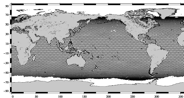
JASON 2 10-day coverage for Jason-2 cycle 77
