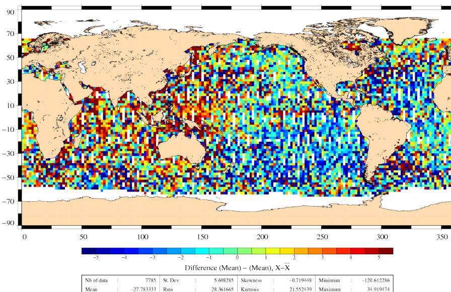
Differences of SLA before orbit error correction J2 – EN (25/07/2010 to 04/08/2010)
