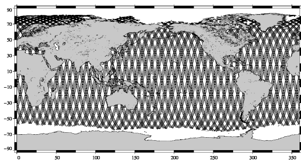
ENVISAT 10-day coverage for Jason-2 cycle 77
