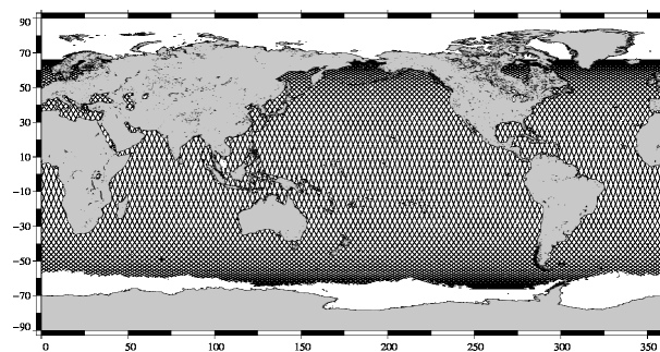
JASON 2 10-day coverage for Jason-2 cycle 78
