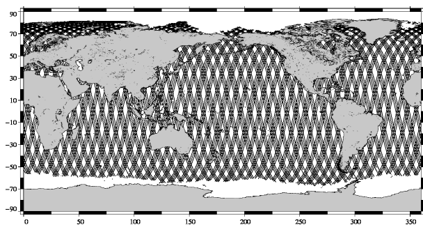
ENVISAT 10-day coverage for Jason-2 cycle 78
