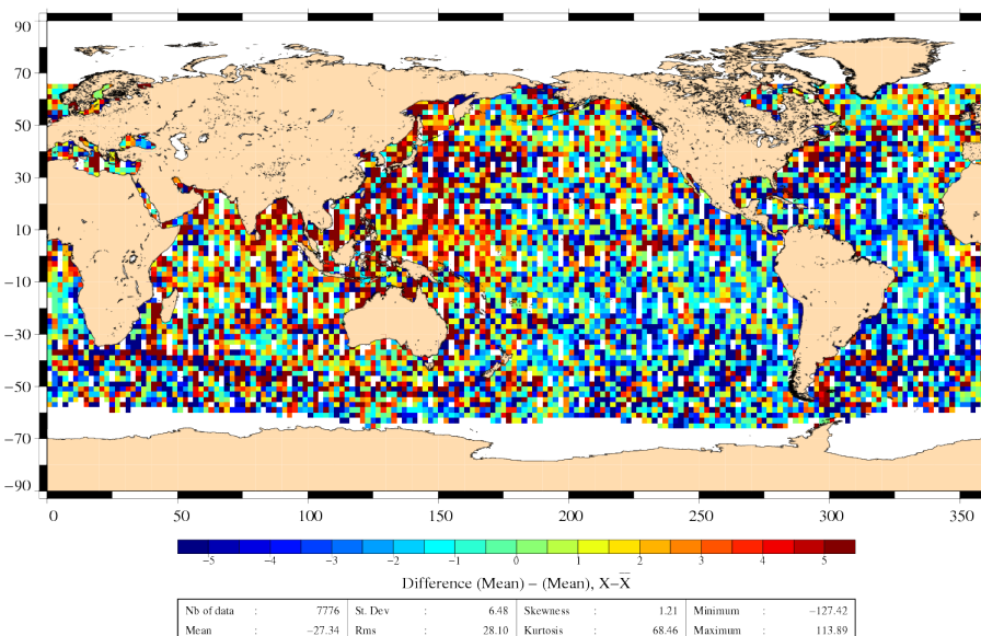
Differences of SLA before orbit error correction J2 – EN (04/08/2010 to 14/08/2010)
