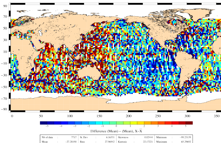
Differences of SLA before orbit error correction J2 – EN (24/08/2010 to 03/09/2010)
