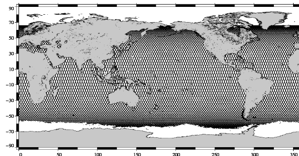
JASON 2 10-day coverage for Jason-2 cycle 080
