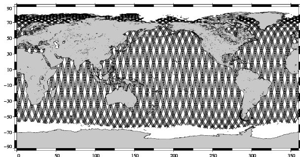
ENVISAT 10-day coverage for Jason-2 cycle 080
