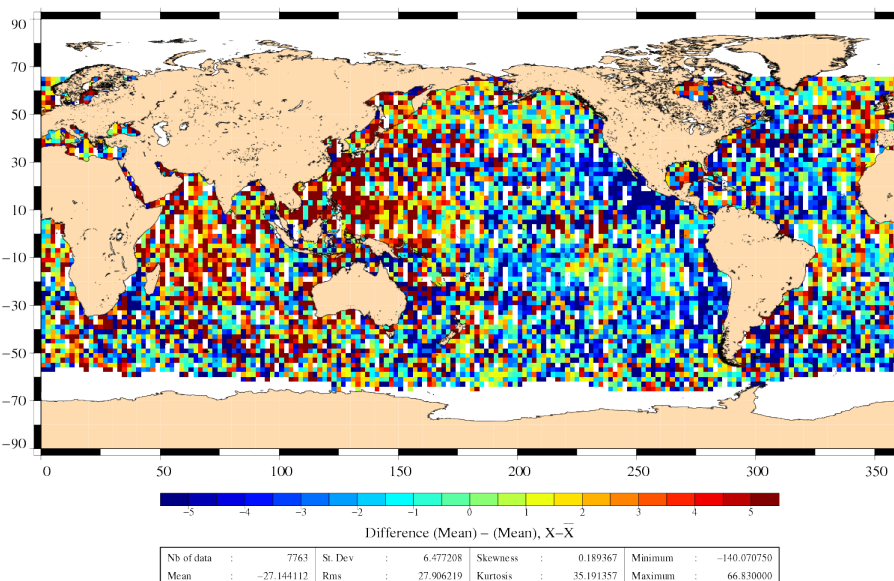
Differences of SLA before orbit error correction J2 – EN (03/09/2010 to 13/09/2010)
