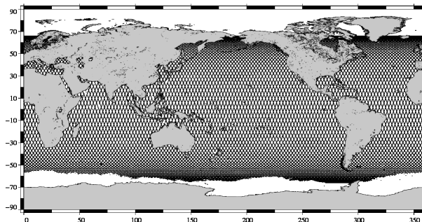
JASON 2 10-day coverage for Jason-2 cycle 085
