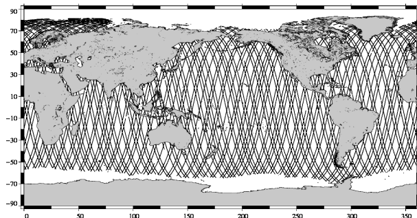
ENVISAT 10-day coverage for Jason-2 cycle 085
