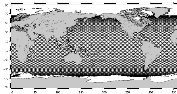
JASON 2 10-day coverage for Jason-2 cycle 090
