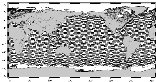
ENVISAT 10-day coverage for Jason-2 cycle 090
