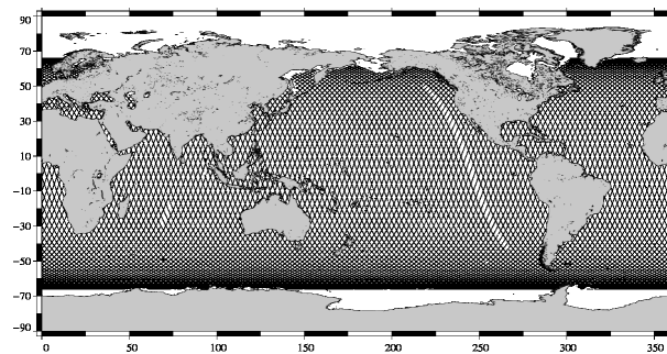
JASON 2 10-day coverage for Jason-2 cycle 094
