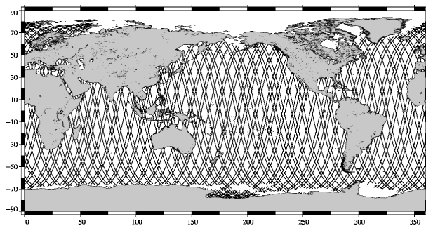
ENVISAT 10-day coverage for Jason-2 cycle 094
