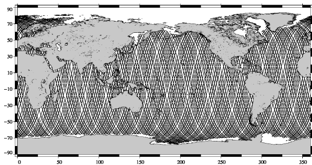
ENVISAT 10-day coverage for Jason-2 cycle 099
