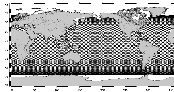
JASON 2 10-day coverage for Jason-2 cycle 099
