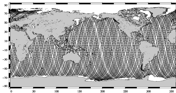
ENVISAT 10-day coverage for Jason-2 cycle 100
