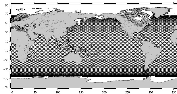
JASON 2 10-day coverage for Jason-2 cycle 100
