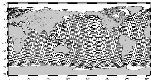
ENVISAT 10-day coverage for Jason-2 cycle 101
