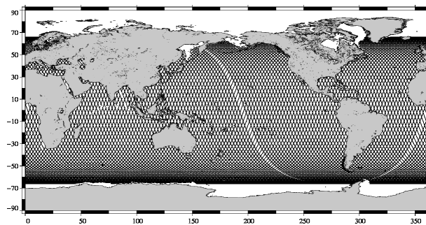
JASON 2 10-day coverage for Jason-2 cycle 101
