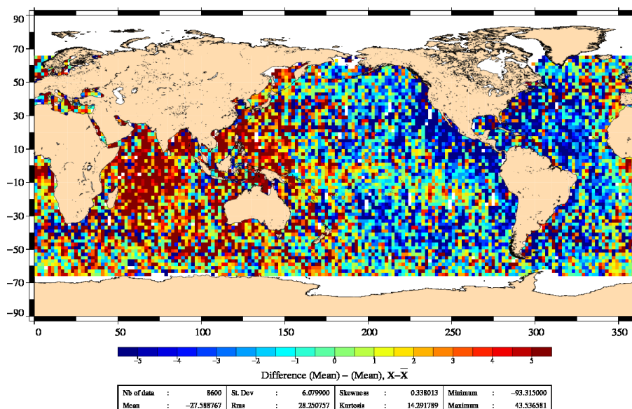
Differences of SLA before orbit error correction J2 – EN (19/04/2011 to 29/04/2011)
