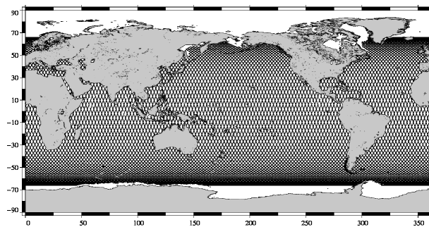
JASON 2 10-day coverage for Jason-2 cycle 103
