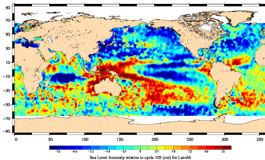
Variability relative to MSS (cm) Cycle 103 EN (19/04/2011 to 29/04/2011)
