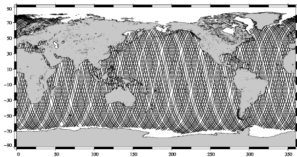
ENVISAT 10-day coverage for Jason-2 cycle 103
