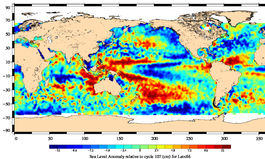
Variability relative to MSS (cm) Cycle 108 EN (08/06/2011 to 17/06/2011)
