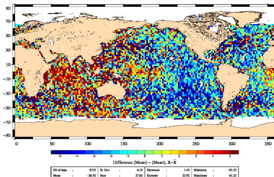
Differences of SLA before orbit error correction J2 – EN (08/06/2011 to 17/06/2011)
