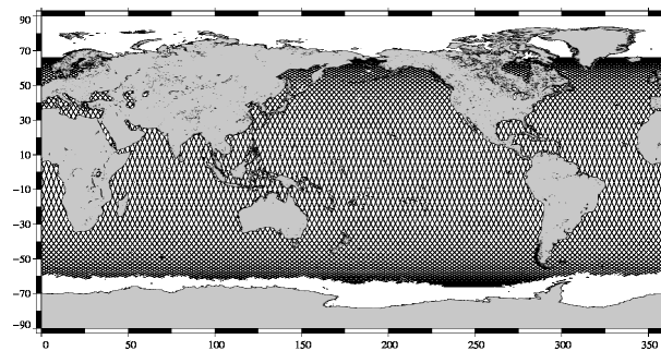
JASON 2 10-day coverage for Jason-2 cycle 113
