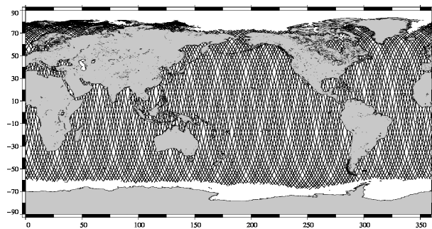
ENVISAT 10-day coverage for Jason-2 cycle 113
