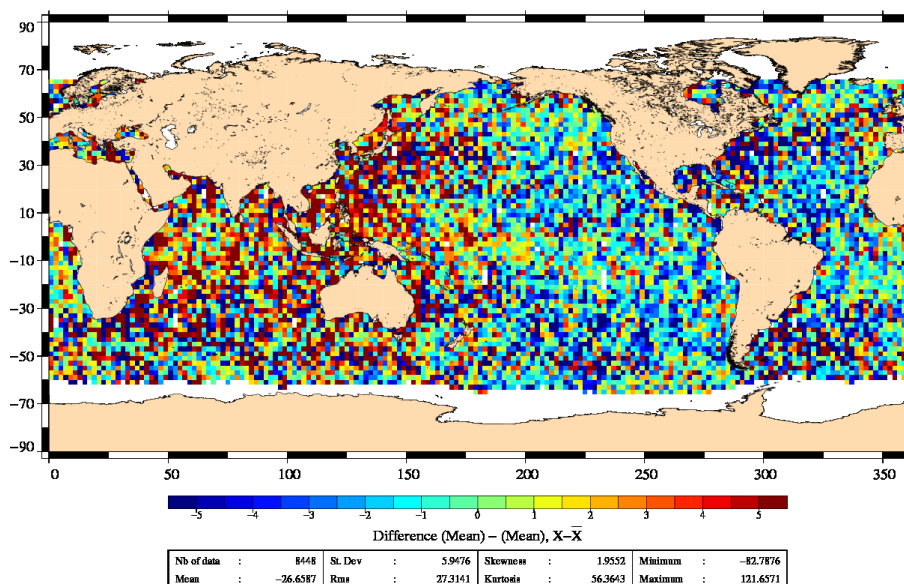
Differences of SLA before orbit error correction J2 – EN (27/07/2011 to 06/08/2011)
