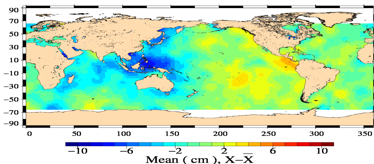
EN/J2 Crossover mean Differences with ECMWF Wet Tropo (cm) (16/08/2011 – 26/08/2011)
