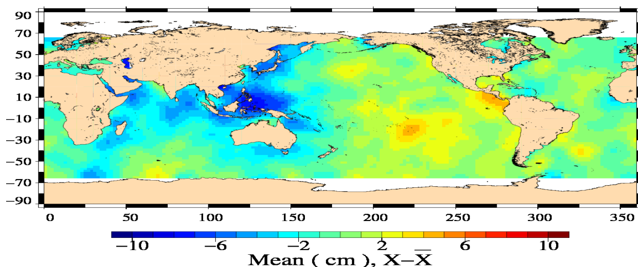
EN/J2 Crossover mean Differences with ECMWF Wet Tropo (cm) (16/08/2011 – 26/08/2011)
