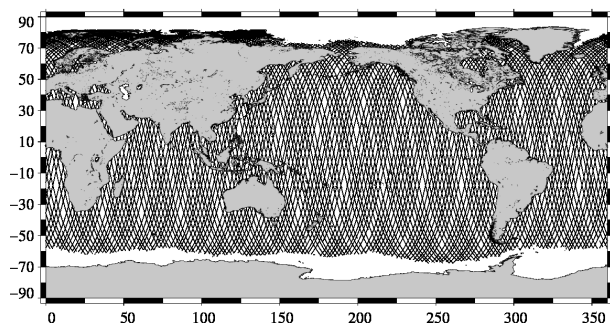
ENVISAT 10-day coverage for Jason-2 cycle 115
