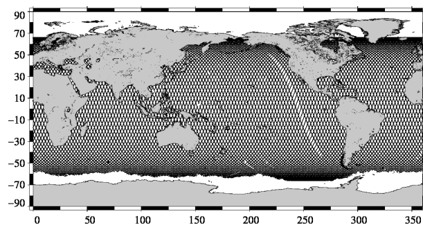
JASON 2 10-day coverage for Jason-2 cycle 115
