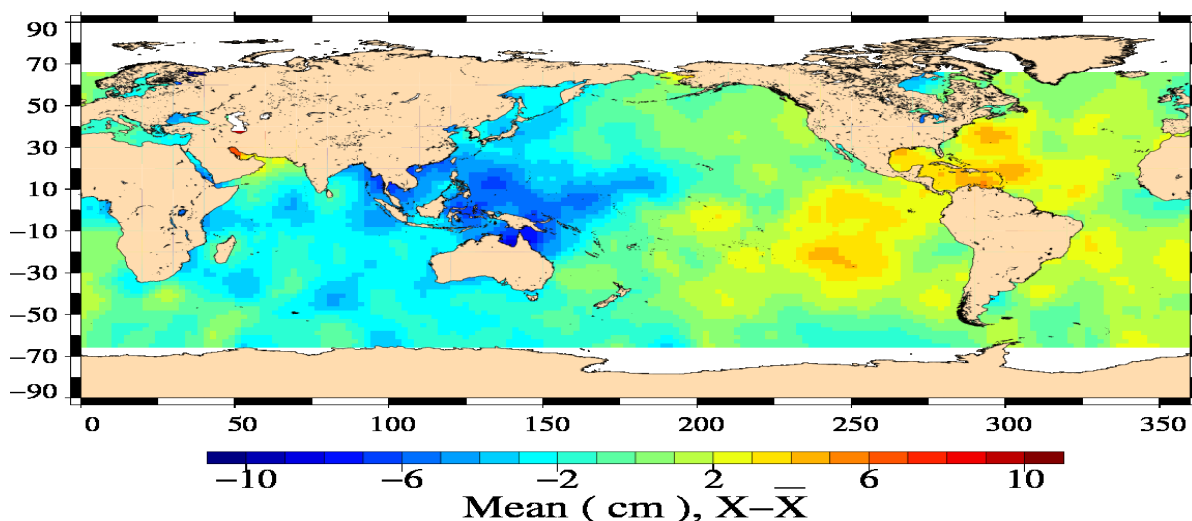
EN/J2 Crossover mean Differences with ECMWF Wet Tropo (cm) (05/09/2011 – 15/09/2011)
