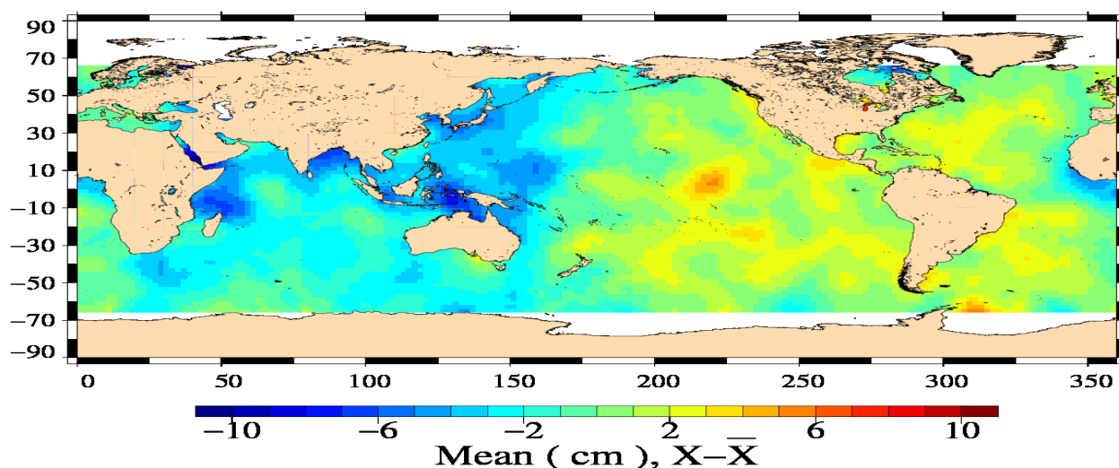
EN/J2 Crossover mean Differences with ECMWF Wet Tropo (cm) (15/09/2011 – 25/09/2011)
