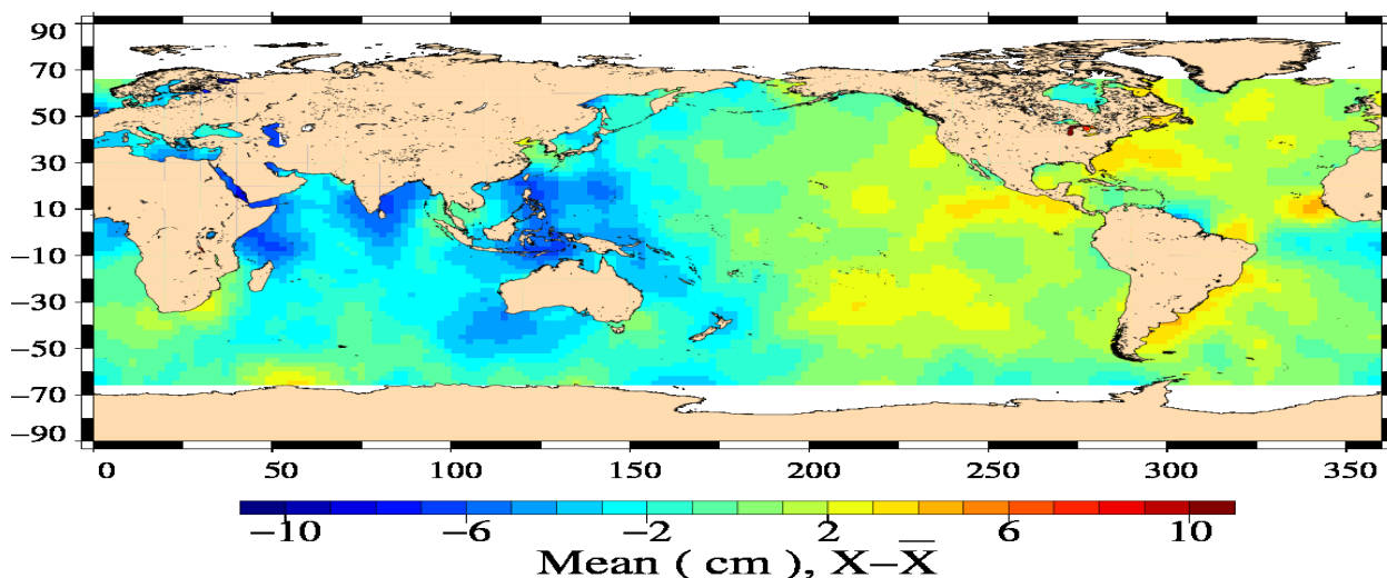
EN/J2 Crossover mean Differences with ECMWF Wet Tropo (cm) (25/09/2011 – 05/10/2011)
