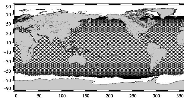
JASON 2 10-day coverage for Jason-2 cycle 119
