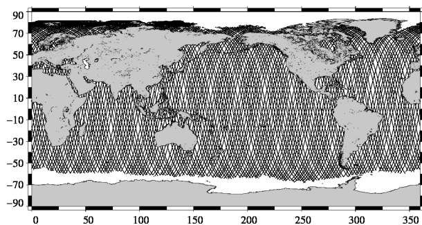
ENVISAT 10-day coverage for Jason-2 cycle 119
