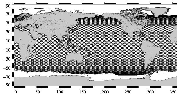
JASON 2 10-day coverage for Jason-2 cycle 120
