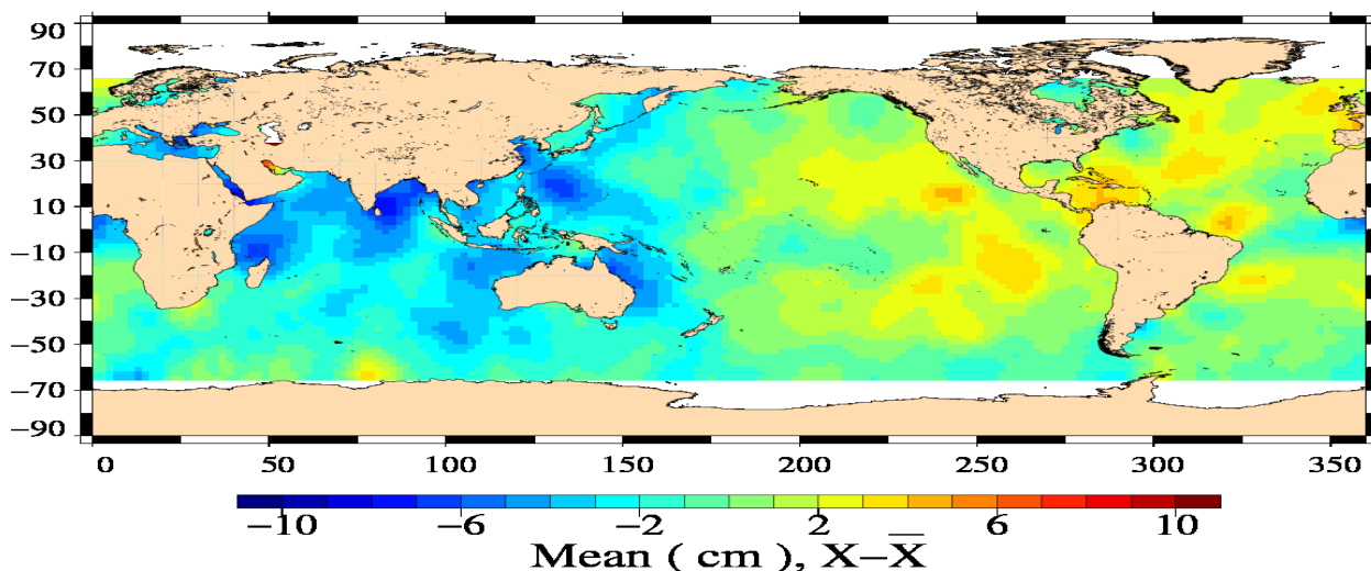
EN/J2 Crossover mean Differences with ECMWF Wet Tropo (cm) (05/10/2011 – 14/10/2011)
