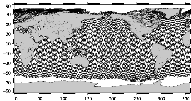
ENVISAT 10-day coverage for Jason-2 cycle 120
