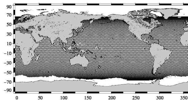
JASON 2 10-day coverage for Jason-2 cycle 121
