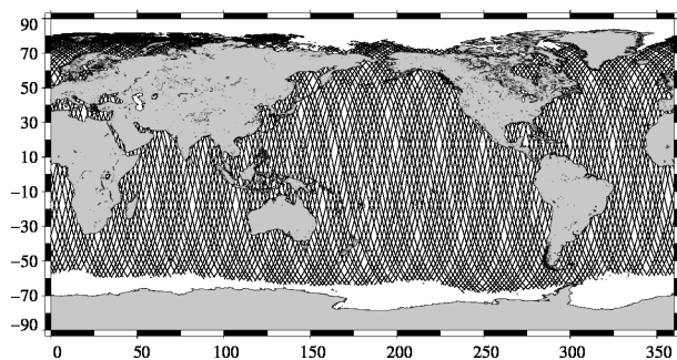
ENVISAT 10-day coverage for Jason-2 cycle 121
