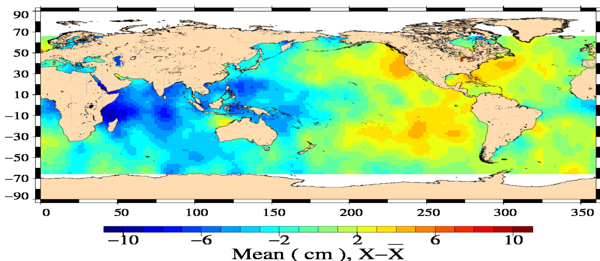
EN/J2 Crossover mean Differences with ECMWF Wet Tropo (cm) (14/10/2011 – 24/10/2011)
