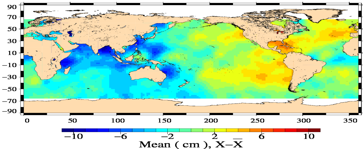
EN/J2 Crossover mean Differences with ECMWF Wet Tropo (cm) (24/10/2011 – 03/11/2011)
