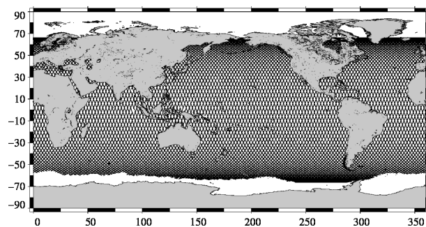
JASON 2 10-day coverage for Jason-2 cycle 122
