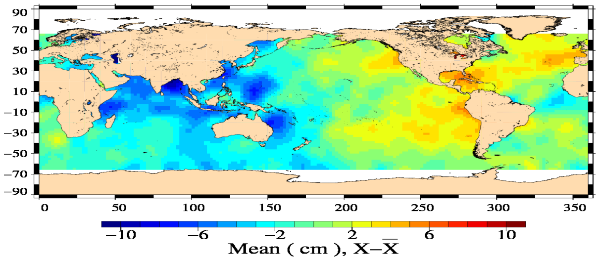
EN/J2 Crossover mean Differences with ECMWF Wet Tropo (cm) (24/10/2011 – 03/11/2011)
