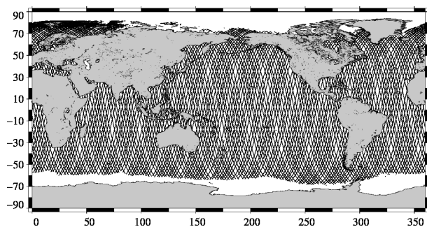
ENVISAT 10-day coverage for Jason-2 cycle 122
