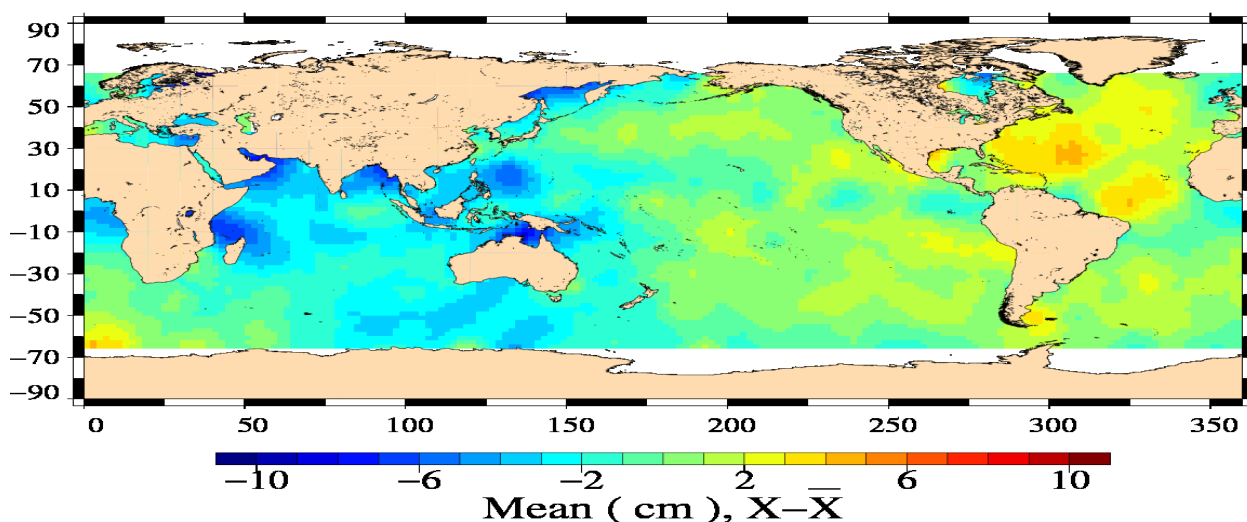
EN/J2 Crossover mean Differences with ECMWF Wet Tropo (cm) (13/11/2011 – 23/11/2011)
