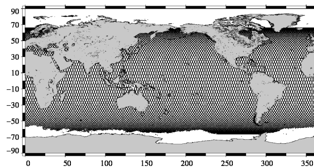
JASON 2 10-day coverage for Jason-2 cycle 124
