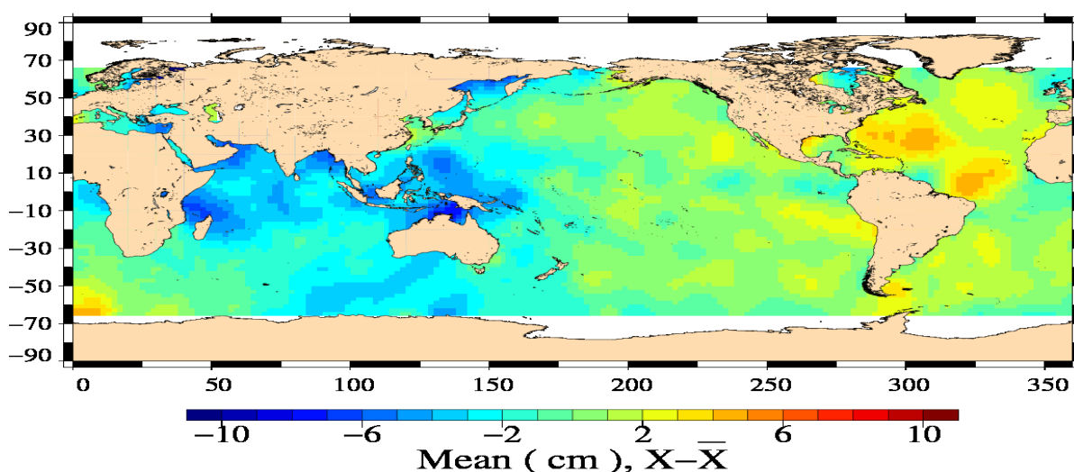
EN/J2 Crossover mean Differences with ECMWF Wet Tropo (cm) (13/11/2011 – 23/11/2011)
