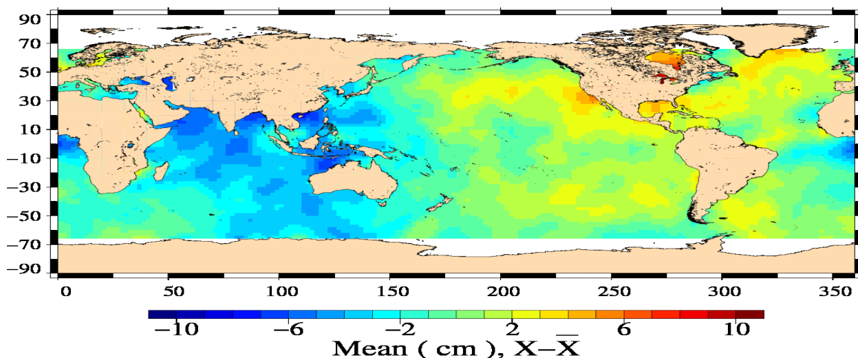
EN/J2 Crossover mean Differences with ECMWF Wet Tropo (cm) (23/11/2011 – 03/12/2011)
