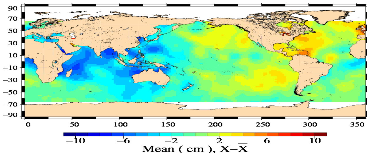
EN/J2 Crossover mean Differences with ECMWF Wet Tropo (cm) (03/12/2011 – 13/12/2011)
