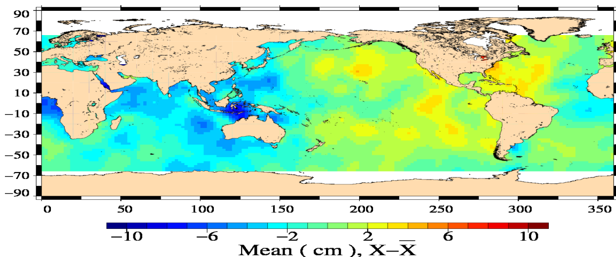
EN/J2 Crossover mean Differences with ECMWF Wet Tropo (cm) (02/01/2012 – 12/01/2012)
