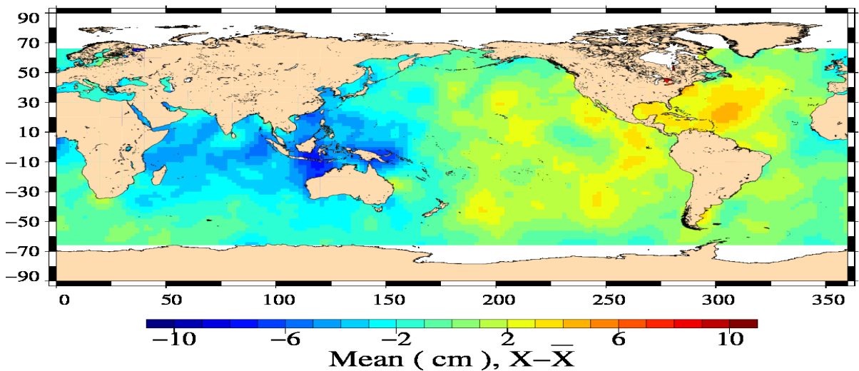
EN/J2 Crossover mean Differences with ECMWF Wet Tropo (cm) (12/01/2012 – 22/01/2012)
