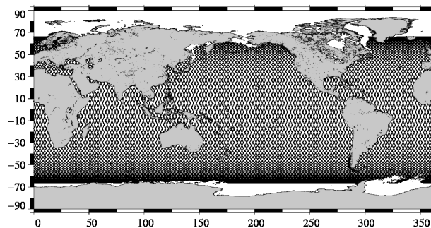
JASON 2 10-day coverage for Jason-2 cycle 130
