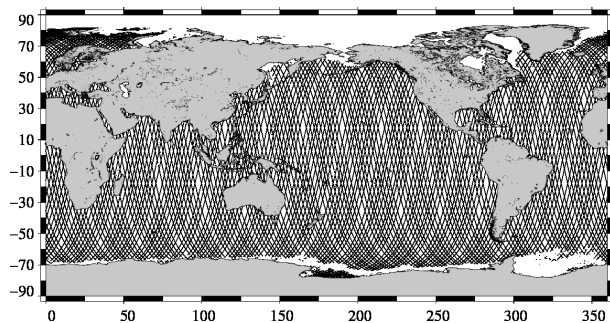
ENVISAT 10-day coverage for Jason-2 cycle 130
