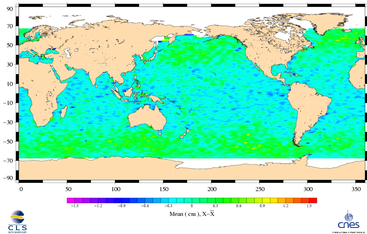
Altimeter ionospheric correction differences Topex (Cycle 347) – Jason (Cycle 004)
