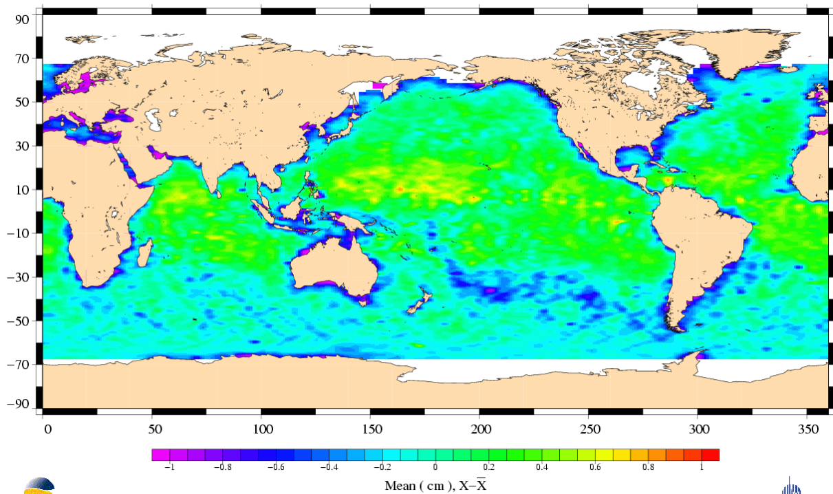
Radiometer correction differences Topex (Cycle 347) – Jason (Cycle 004)
