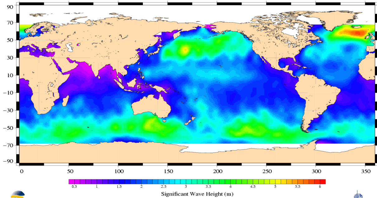
Jason-1 Cycle 004 13/02/2002 – 23/02/2002
