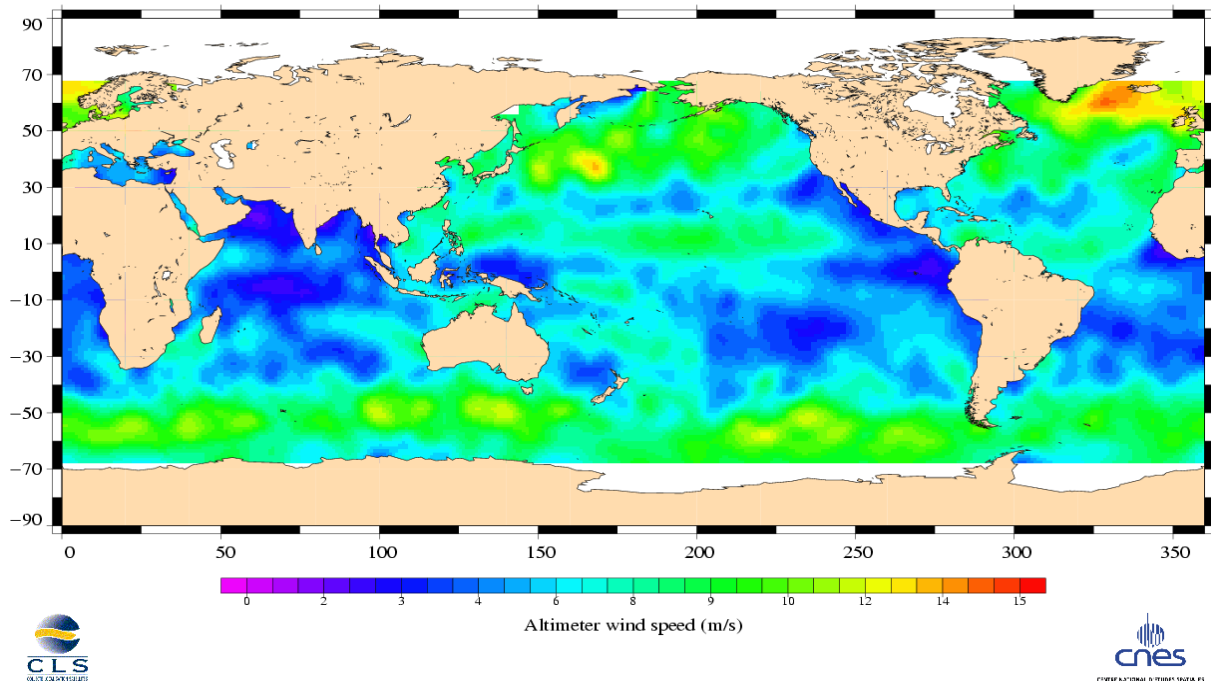
Jason-1 Cycle 004 13/02/2002 – 23/02/2002
