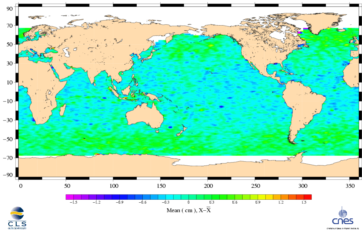
Altimeter ionospheric correction differences Topex (Cycle 348) – Jason (Cycle 005)
