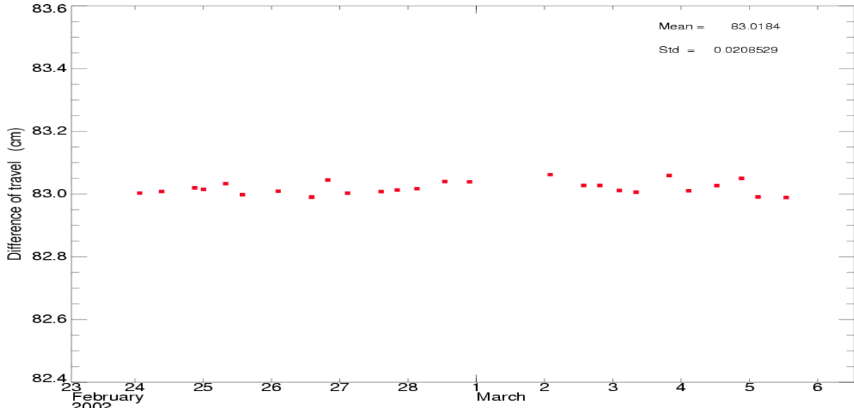
Difference of travel between E and R lines of the PTR in Ku band
