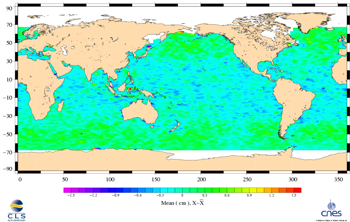
Altimeter ionospheric correction differences Topex (Cycle 349) – Jason (Cycle 006)
