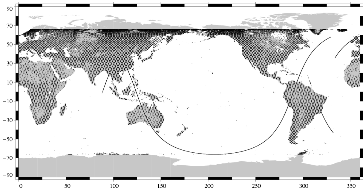
Missing measurements Jason-1 Cycle 006 (05/03/2002 / 15/03/2002)
