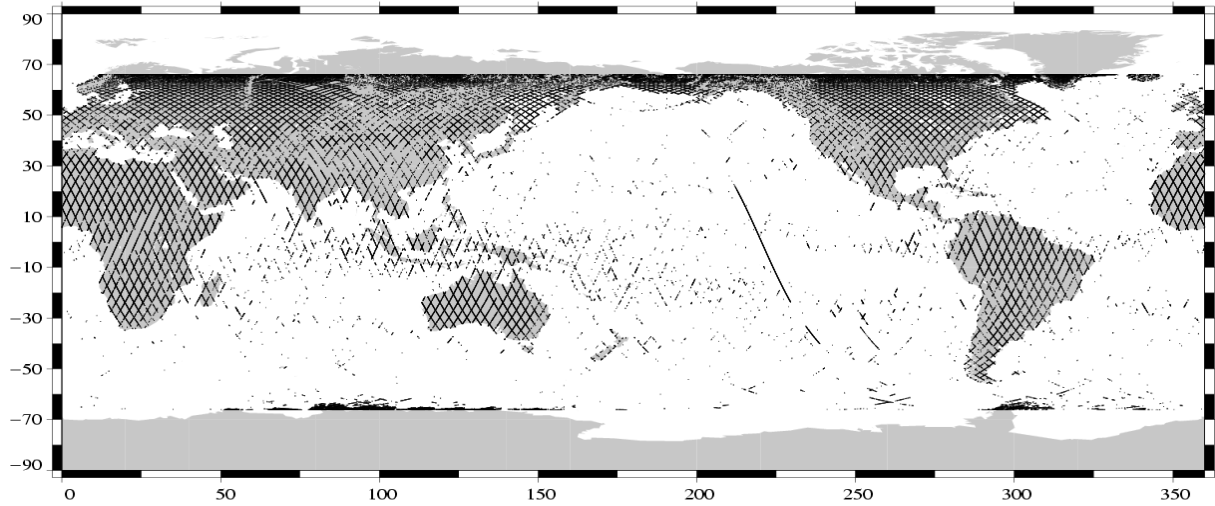
Edited measurements Jason-1 Cycle 006 (05/03/2002 / 15/03/2002)
