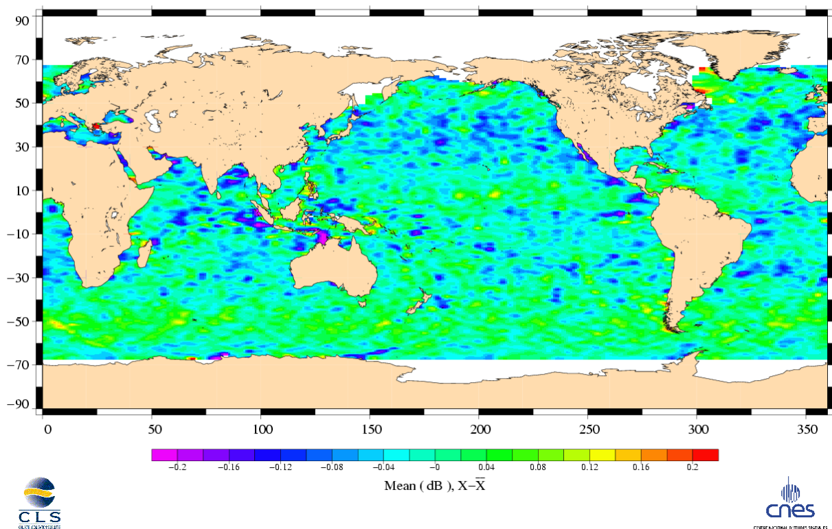
Ku SIGMA0 differences Topex (Cycle 349) – Jason (Cycle 006)
