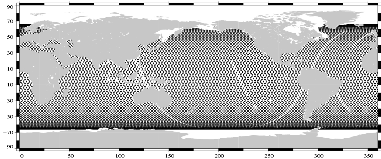
Valid data Jason-1 Cycle 006 (05/03/2002 / 15/03/2002)
