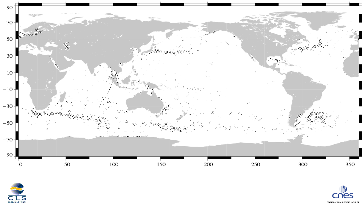
(SSH – MSS) differences greater than 30 cm Jason / Cycle 006
