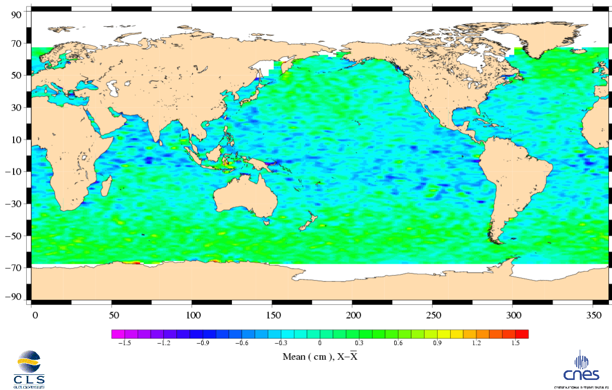
Altimeter ionospheric correction differences Topex (Cycle 351) – Jason (Cycle 008)
