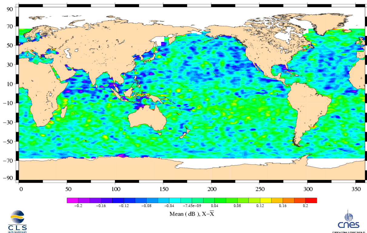
Ku SIGMA0 differences Topex (Cycle 351) – Jason (Cycle 008)
