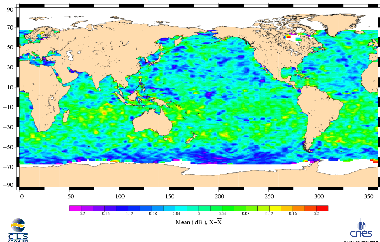
Ku SIGMA0 differences Topex (Cycle 358) – Jason (Cycle 015)
