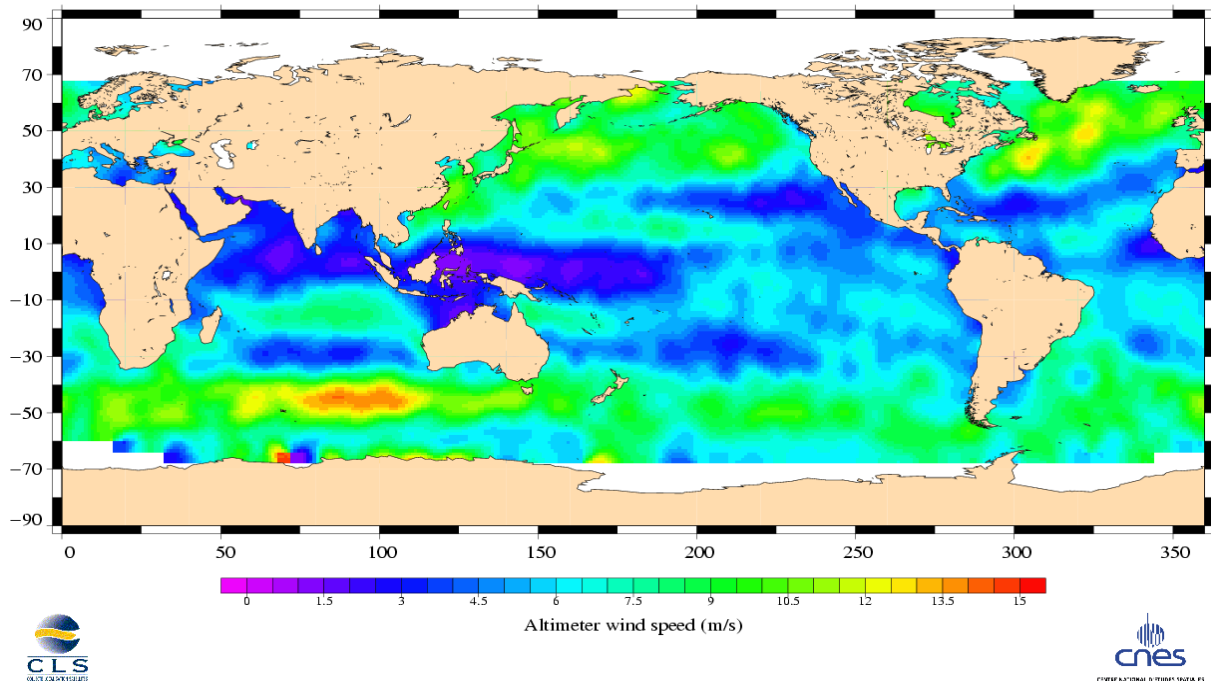
Jason-1 Cycle 030 29/10/2002 – 08/11/2002
