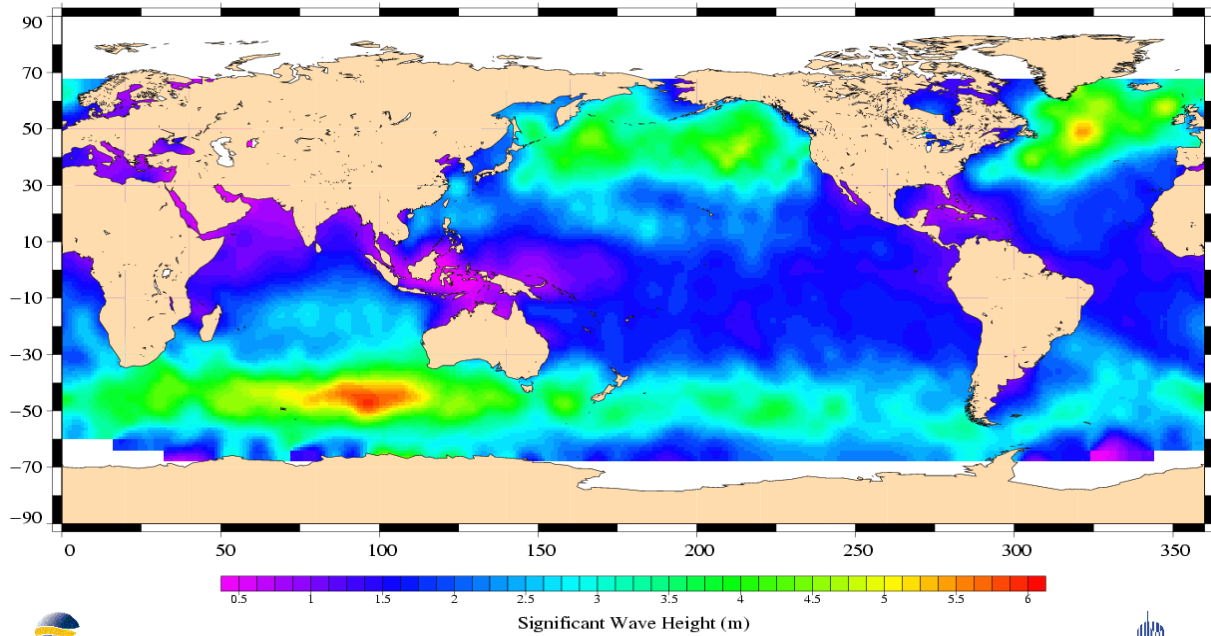
Jason-1 Cycle 030 29/10/2002 – 08/11/2002
