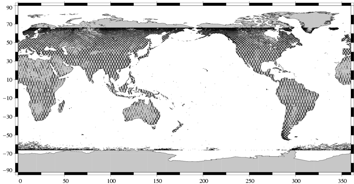
Missing measurements Jason-1 Cycle 030 (29/10/2002 / 08/11/2002)
