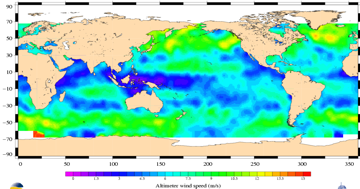
Jason-1 Cycle 031 08/11/2002 – 18/11/2002
