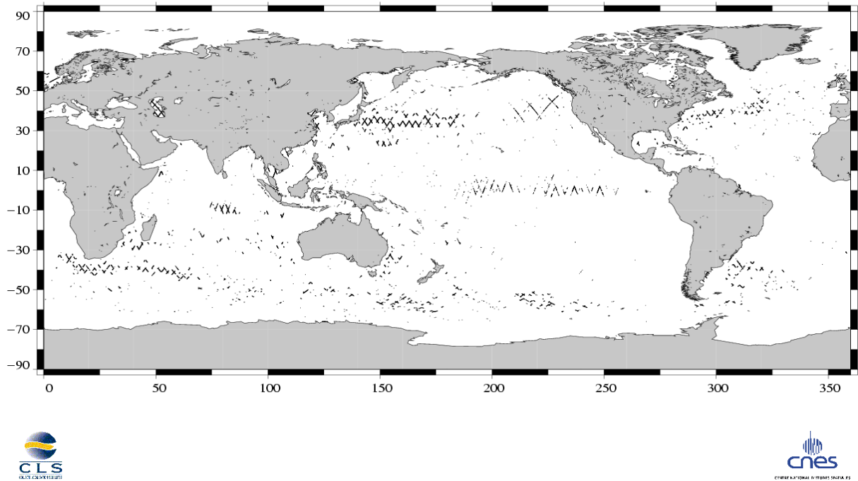
(SSH – MSS) differences greater than 30 cm Jason / Cycle 031
