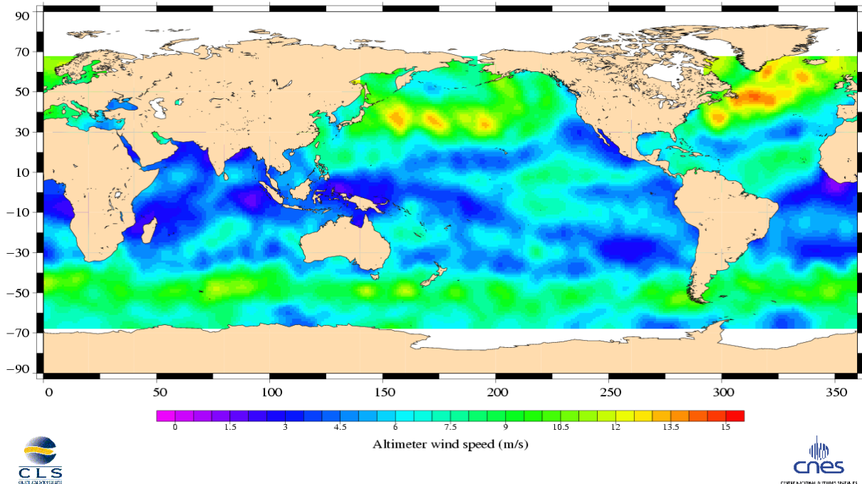
Jason-1 Cycle 038 17/01/2003 – 27/01/2003
