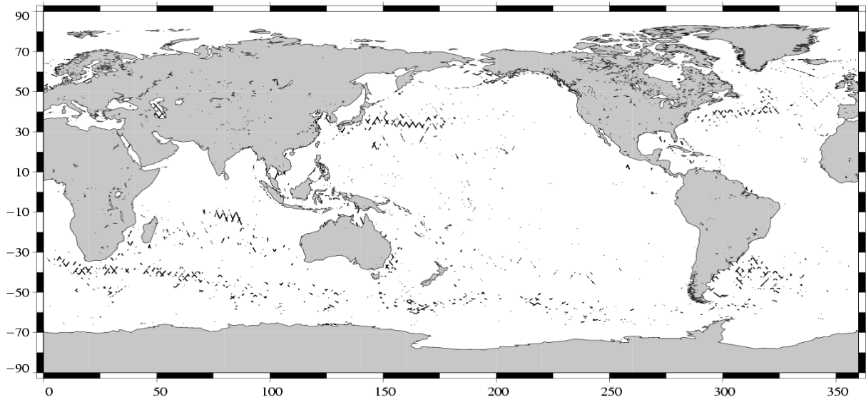
(SSH – MSS) differences greater than 30 cm Jason / Cycle 038
