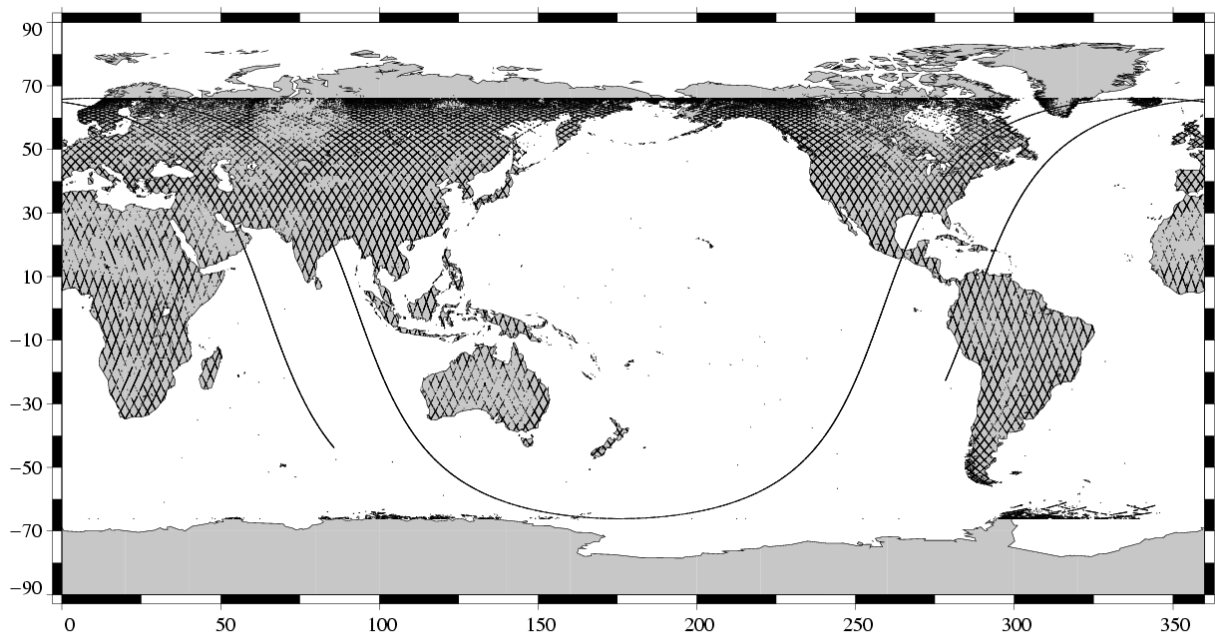
Missing measurements Jason-1 Cycle 038 (17/01/2003 / 27/01/2003)
