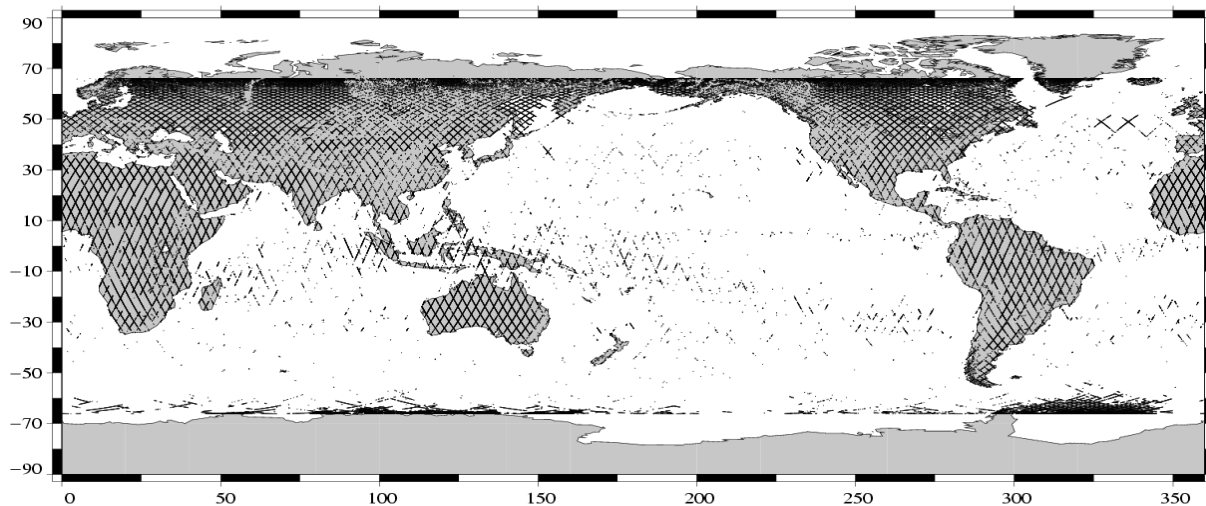
Edited measurements Jason-1 Cycle 038 (17/01/2003 / 27/01/2003)
