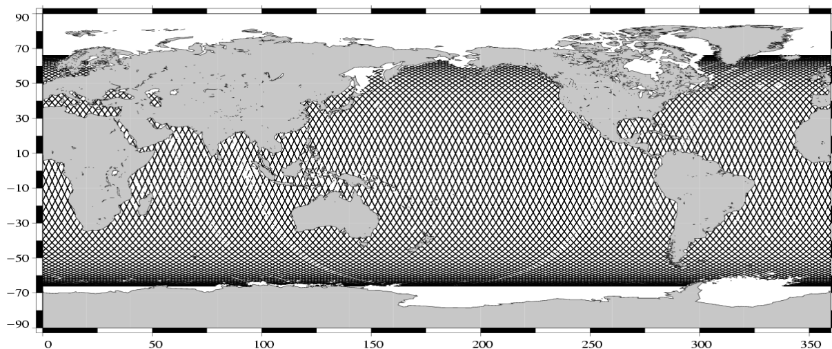
Valid data Jason-1 Cycle 038 (17/01/2003 / 27/01/2003)
