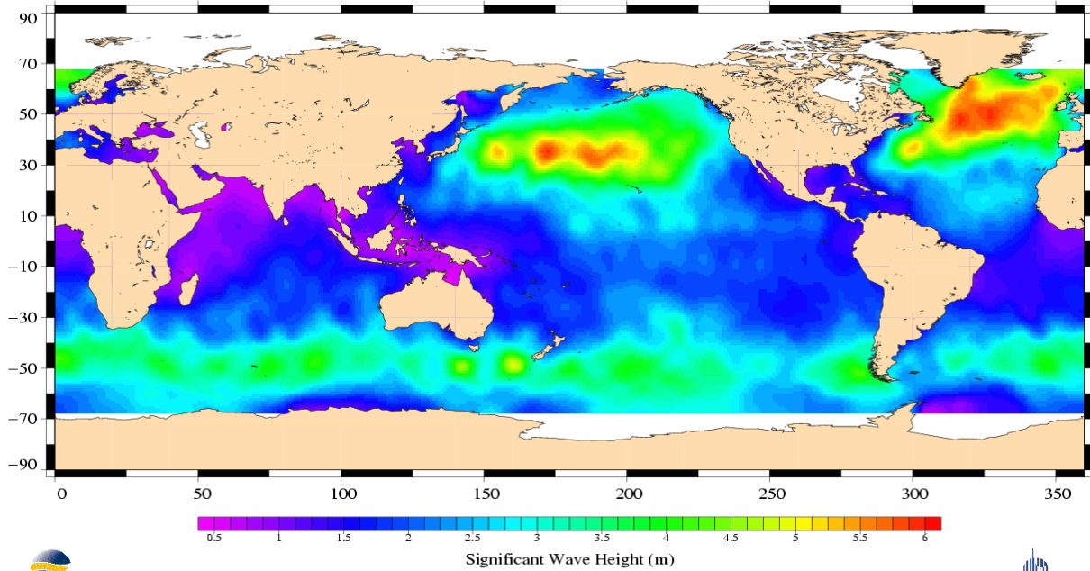
Jason-1 Cycle 038 17/01/2003 – 27/01/2003
