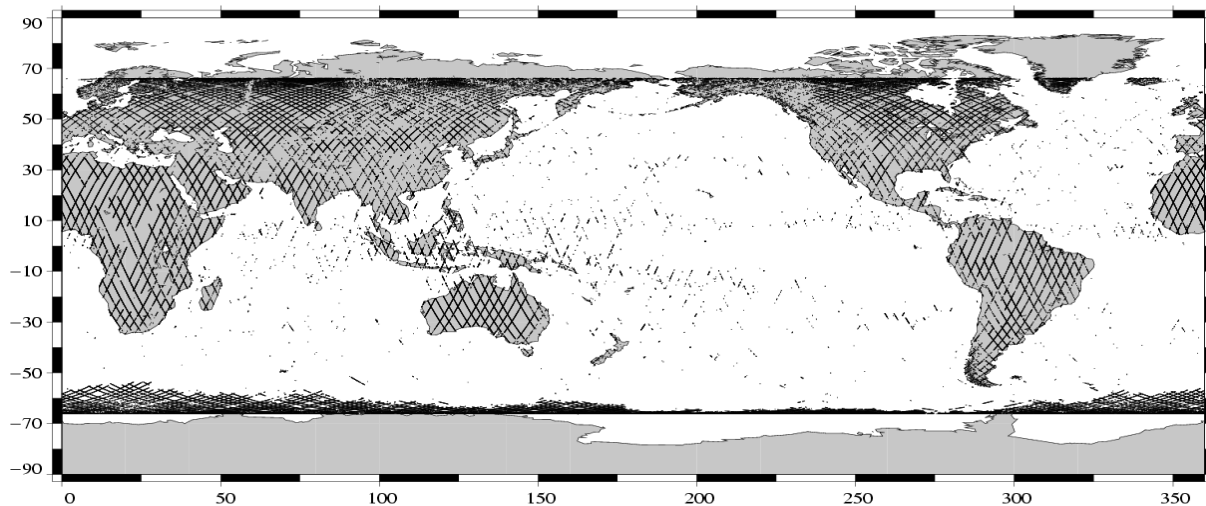
Edited measurements Jason-1 Cycle 068 (10/11/2003 / 18/11/2003)
