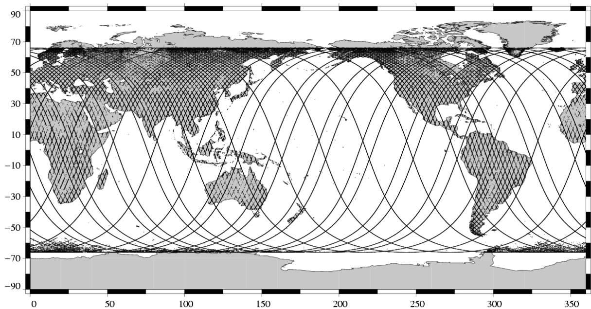
Missing measurements Jason-1 Cycle 068 (10/11/2003 / 18/11/2003)
