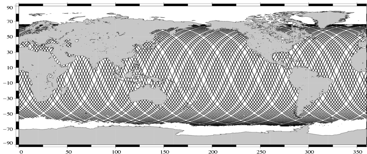
Valid data Jason-1 Cycle 068 (10/11/2003 / 18/11/2003)
