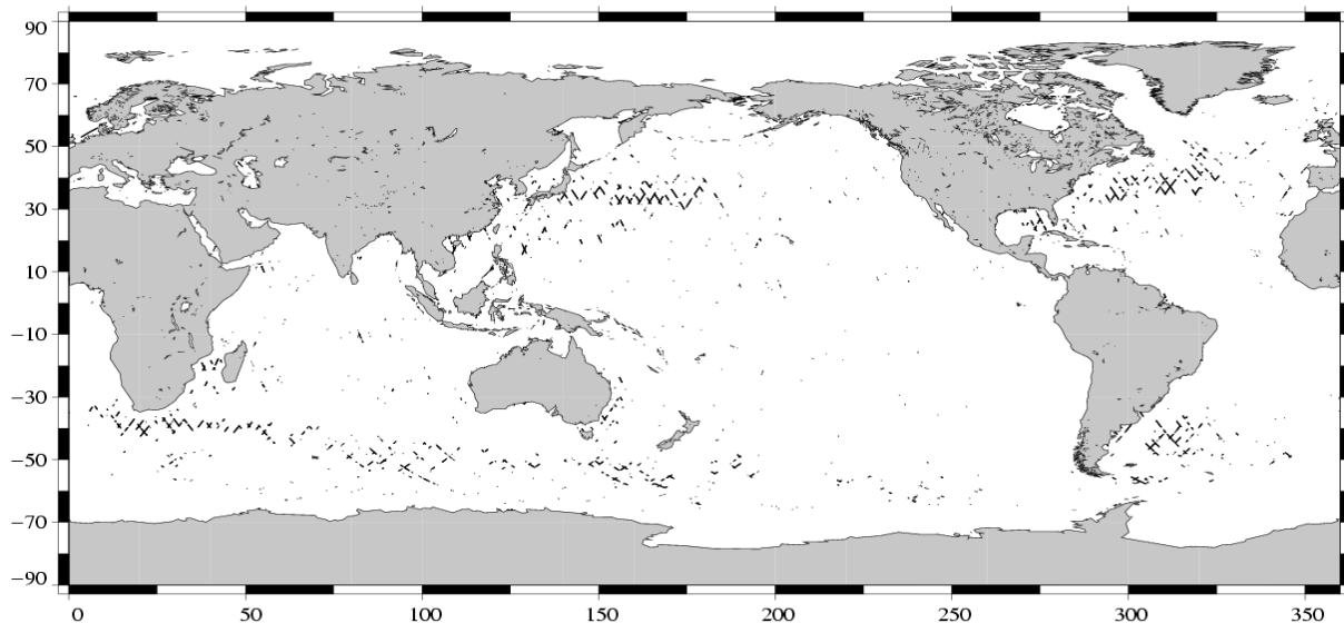
(SSH – MSS) differences greater than 30 cm Jason / Cycle 068
