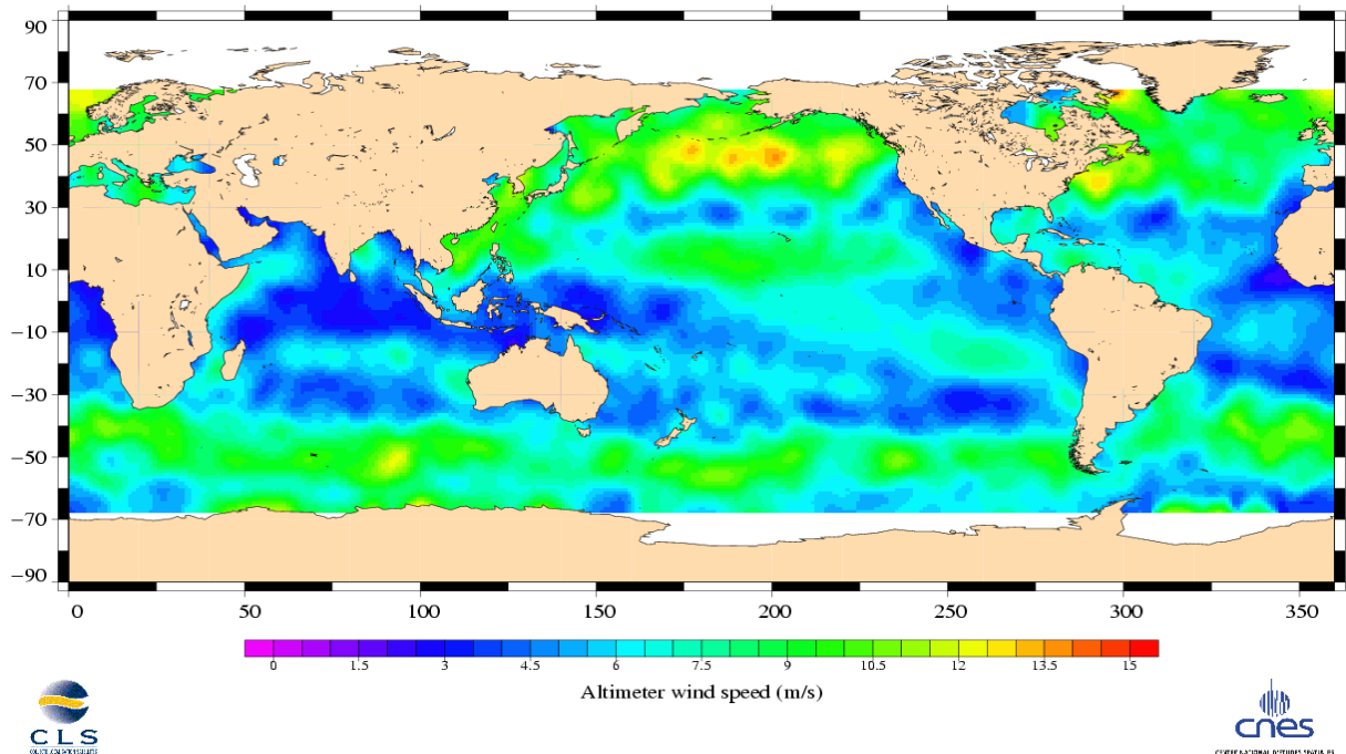
Jason-1 Cycle 071 10/12/2003 – 20/12/2003
