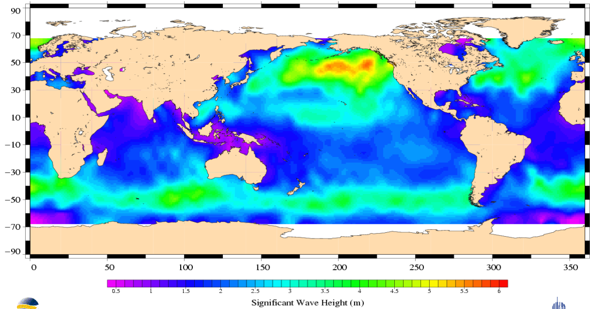
Jason-1 Cycle 071 10/12/2003 – 20/12/2003
