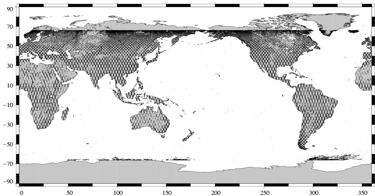
Missing measurements Jason-1 Cycle 073 (30/12/2003 / 09/01/2004)
