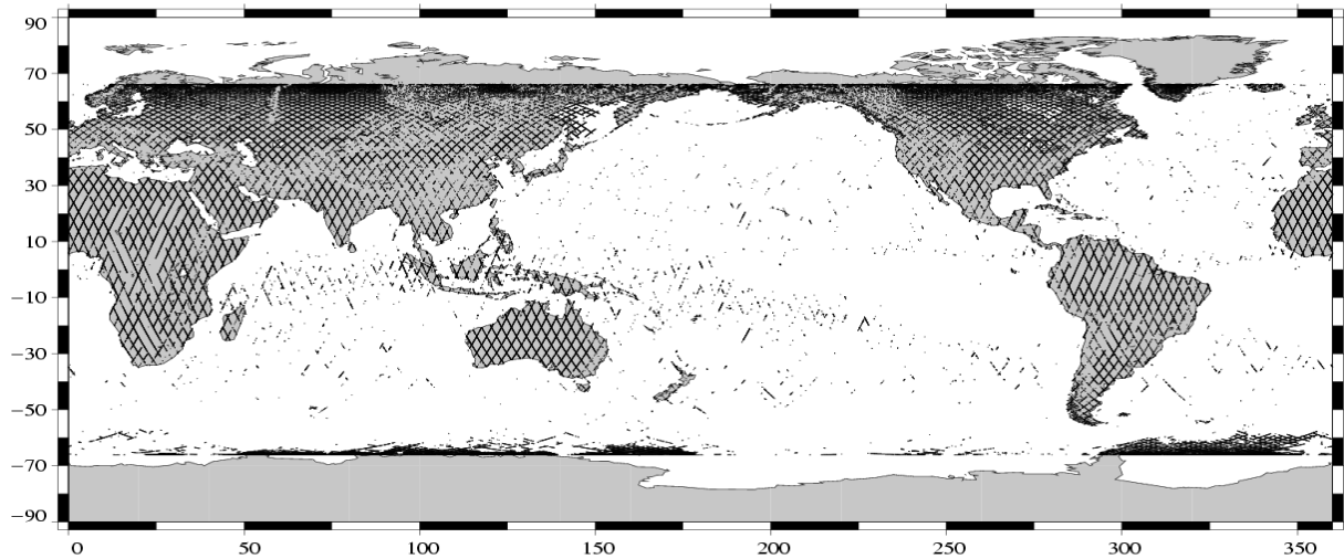
Edited measurements Jason-1 Cycle 073 (30/12/2003 / 09/01/2004)
