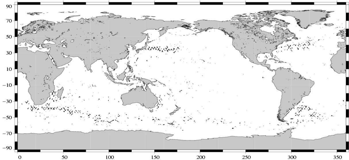
(SSH – MSS) differences greater than 30 cm Jason / Cycle 073
