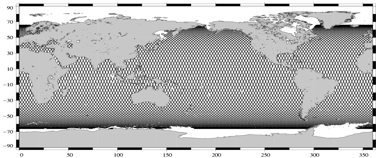
Valid data Jason-1 Cycle 073 (30/12/2003 / 09/01/2004)
