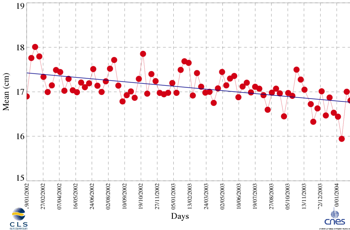
Mean Sea Level
