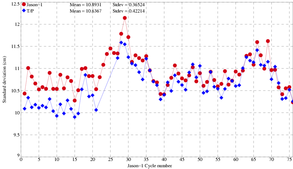
Standard deviation of SLA Residuals
