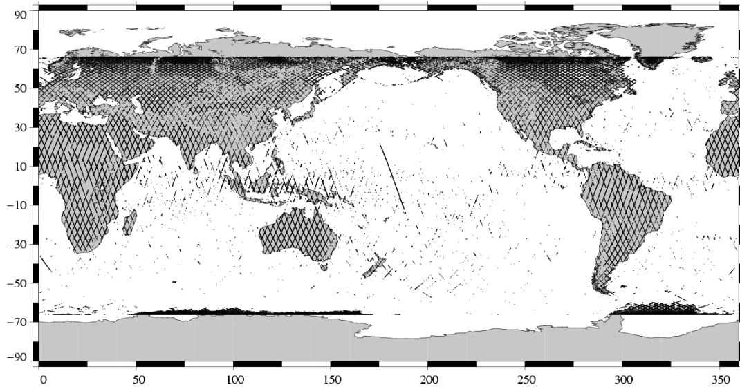
Edited measurements Jason-1 Cycle 084 (17/04/2004 / 27/04/2004)
