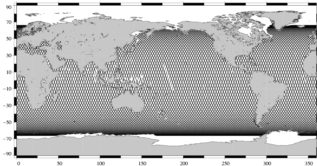
Valid data Jason-1 Cycle 084 (17/04/2004 / 27/04/2004)
