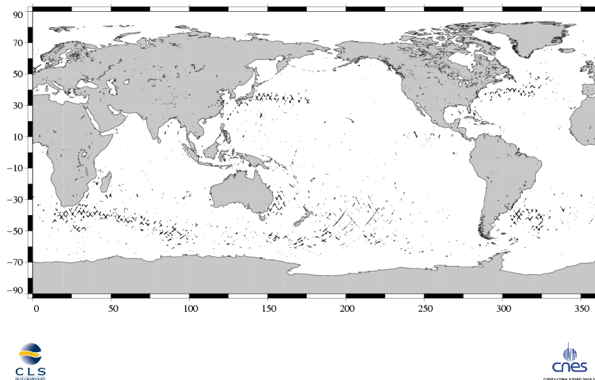
(SSH – MSS) differences greater than 30 cm Jason / Cycle 084
