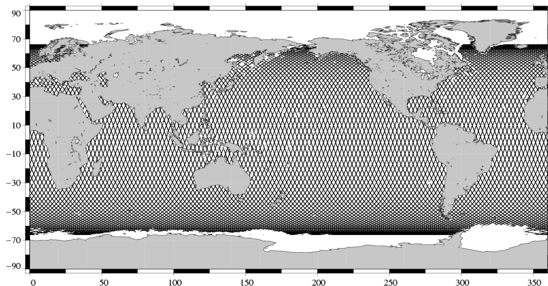
Valid data Jason-1 Cycle 087 (16/05/2004 / 26/05/2004)
