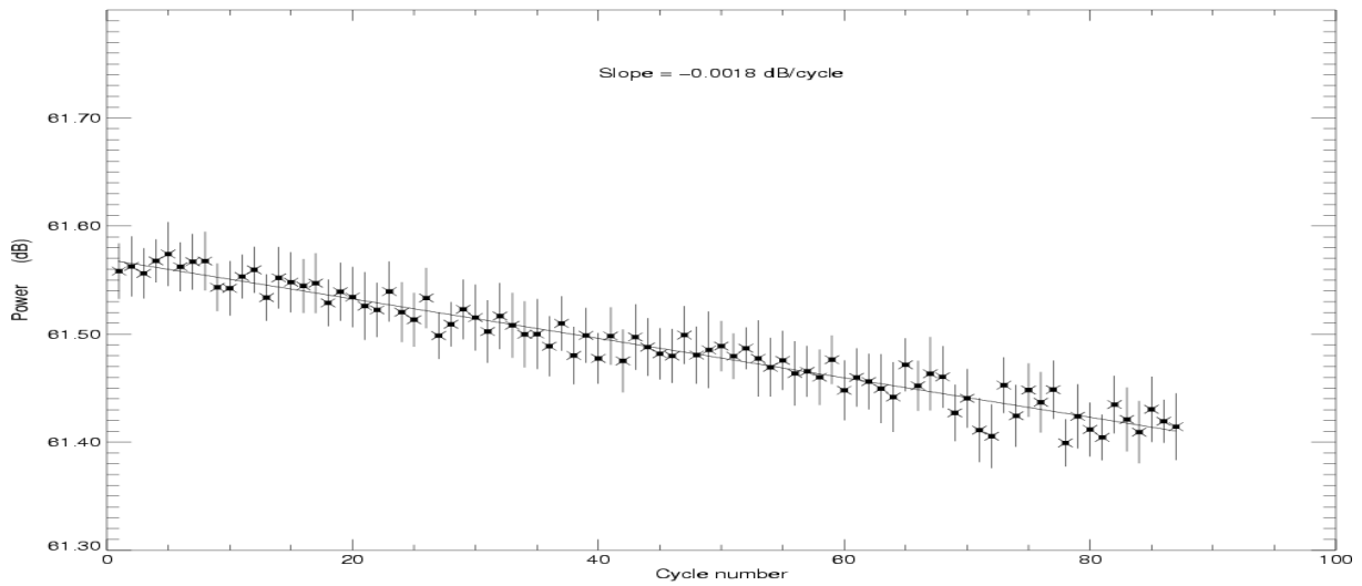
POSEIDON2 – Cycle 087
