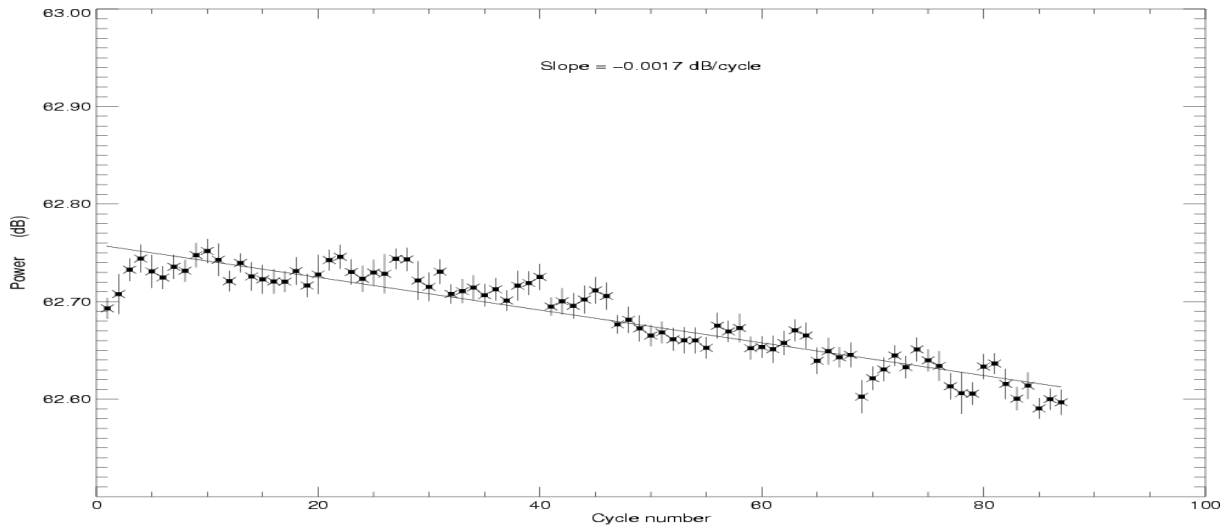
POSEIDON2 – Cycle 087
