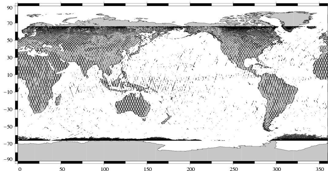
Edited measurements Jason-1 Cycle 087 (16/05/2004 / 26/05/2004)
