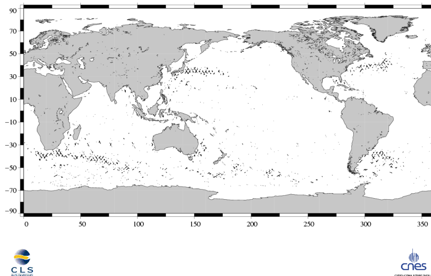
(SSH – MSS) differences greater than 30 cm Jason / Cycle 087
