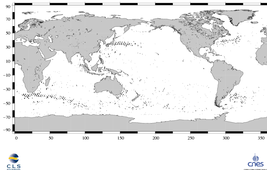
(SSH – MSS) differences greater than 30 cm Jason / Cycle 088
