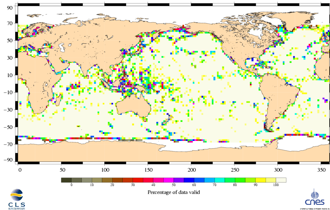
Percentage of valid data relative to the nominal pass Jason-1 Cycle 088 (26/05/2004 / 05/06/2004)
