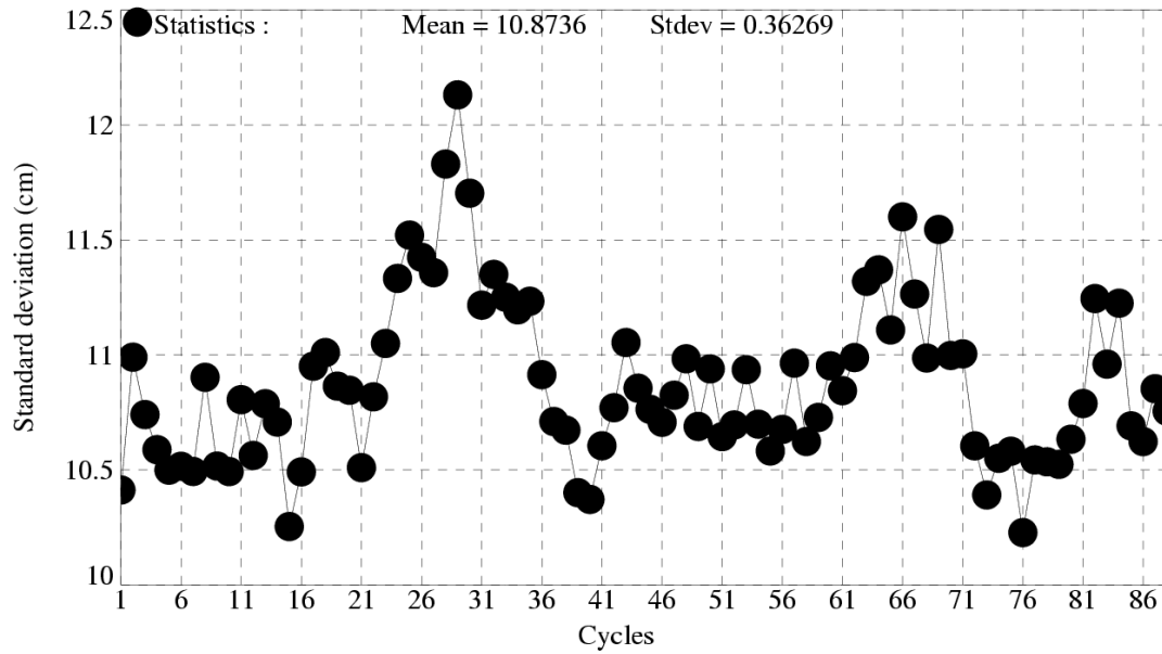
Standard deviation of Sea Level Anomalies
