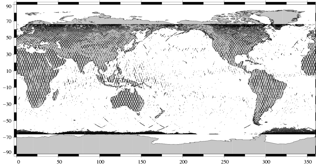
Edited measurements Jason-1 Cycle 088 (26/05/2004 / 05/06/2004)
