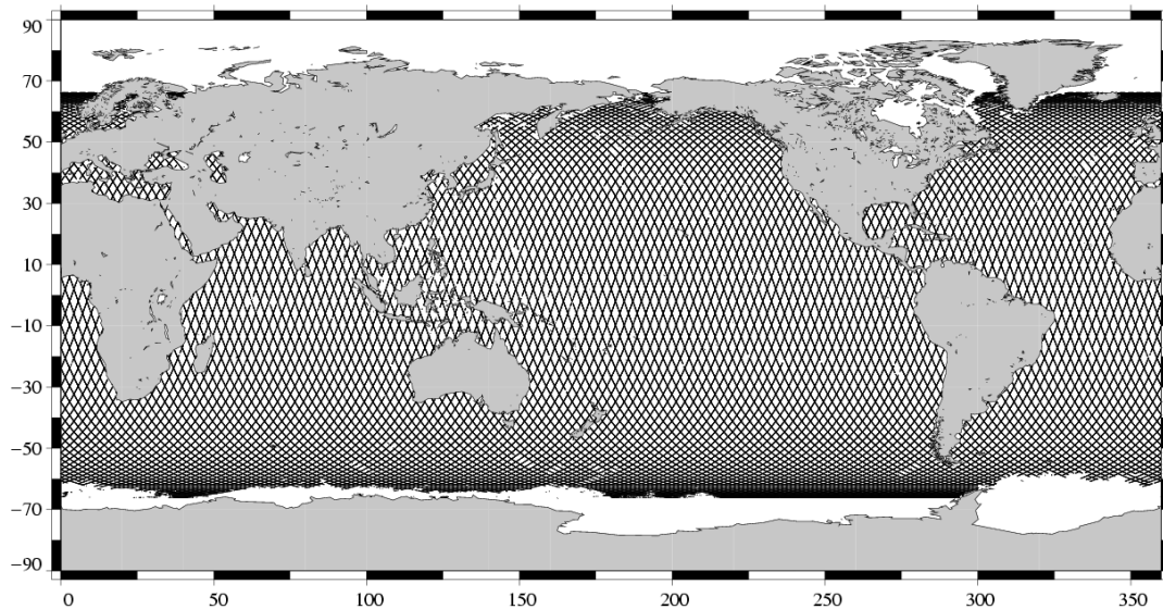
Valid data Jason-1 Cycle 088 (26/05/2004 / 05/06/2004)
