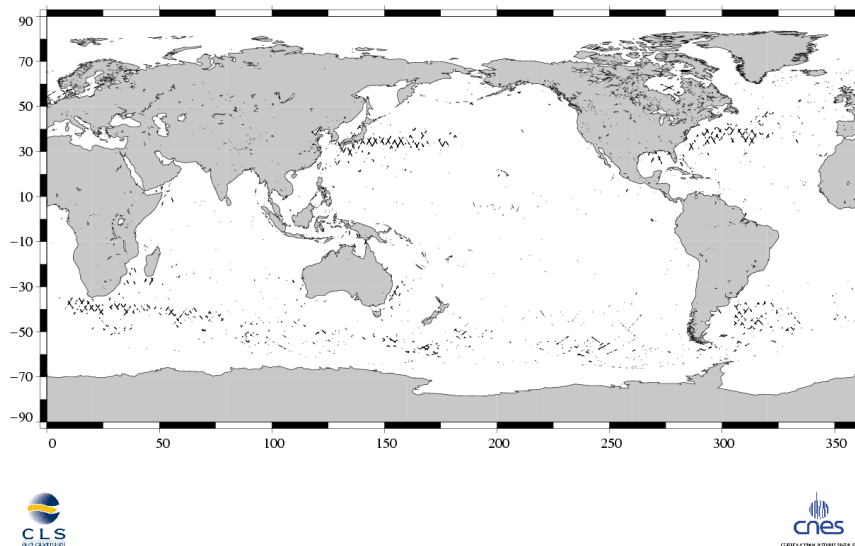
(SSH – MSS) differences greater than 30 cm Jason / Cycle 099
