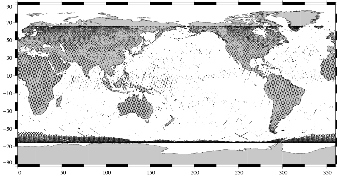
Edited measurements Jason-1 Cycle 099 (12/09/2004 / 22/09/2004)
