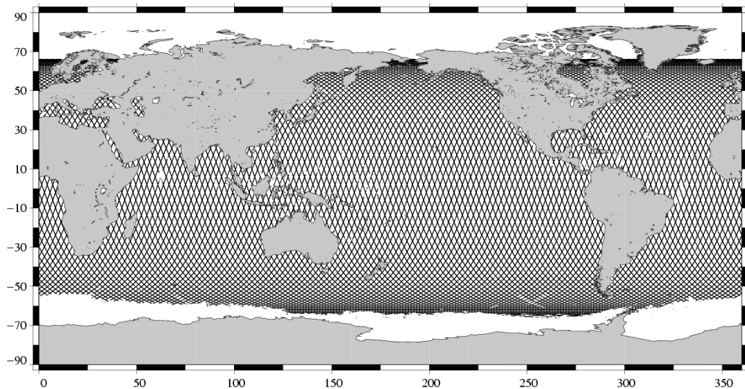
Valid data Jason-1 Cycle 099 (12/09/2004 / 22/09/2004)
