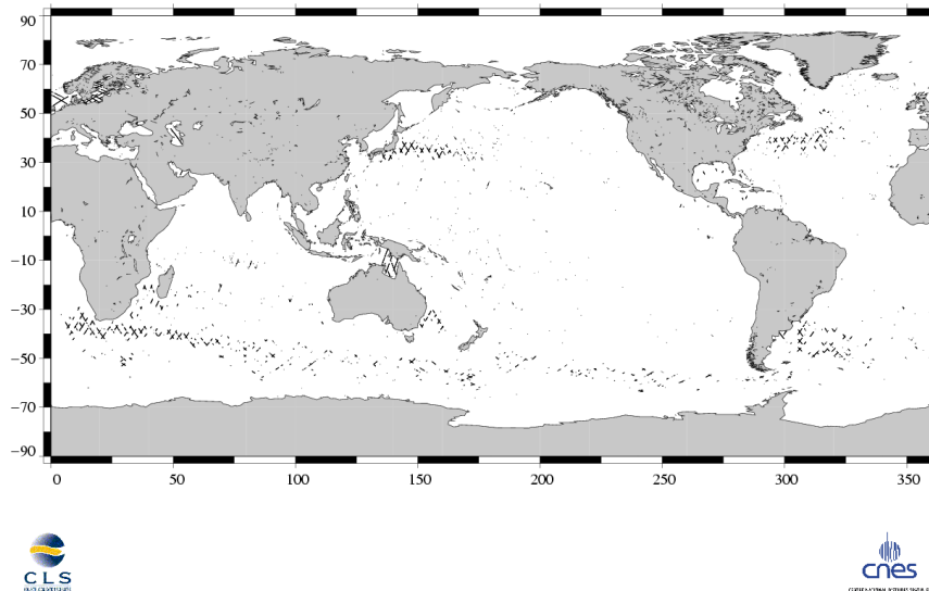
(SSH – MSS) differences greater than 30 cm Jason / Cycle 112
