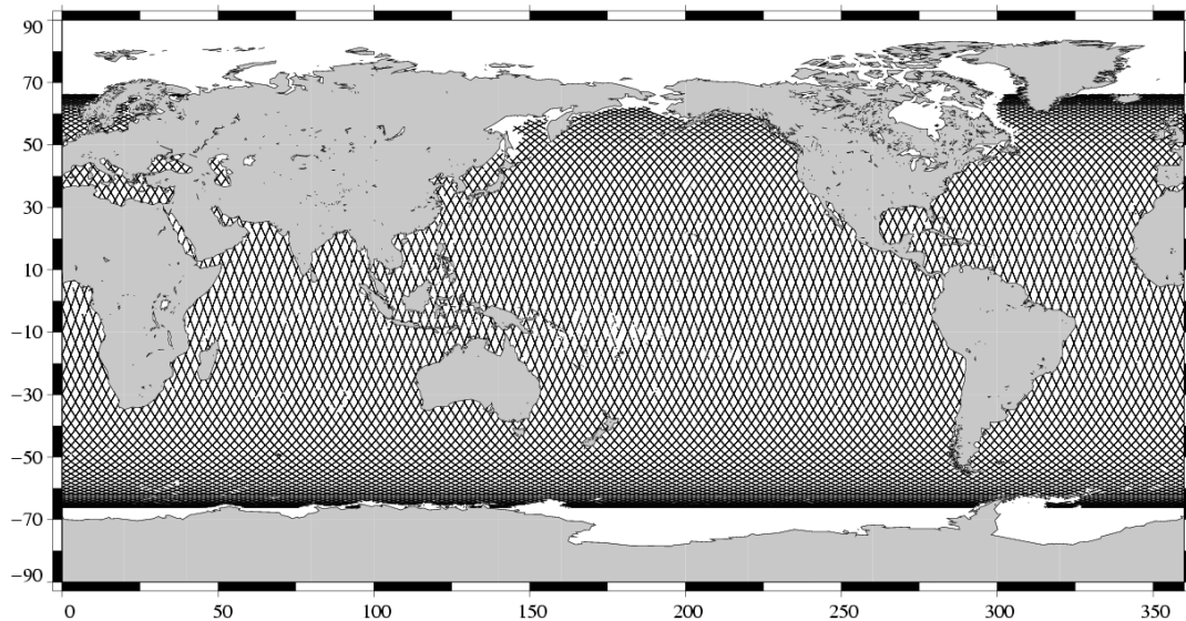
Valid data Jason-1 Cycle 112 (19/01/2005 / 29/01/2005)
