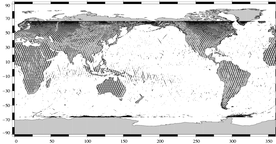
Edited measurements Jason-1 Cycle 112 (19/01/2005 / 29/01/2005)
