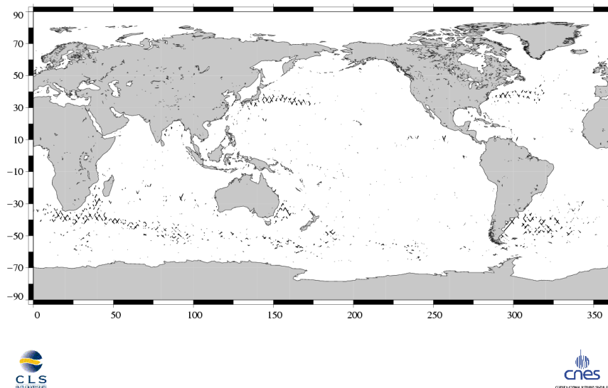
(SSH – MSS) differences greater than 30 cm Jason / Cycle 121
