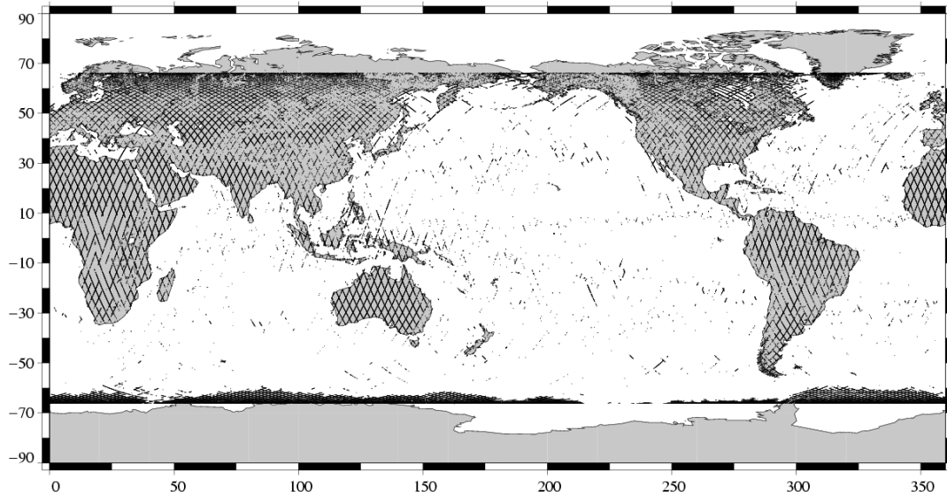
Edited measurements Jason-1 Cycle 126 (07/06/2005 / 17/06/2005)
