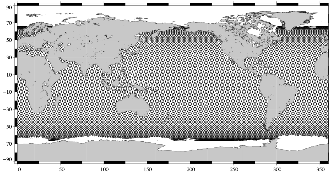
Valid data Jason-1 Cycle 126 (07/06/2005 / 17/06/2005)
