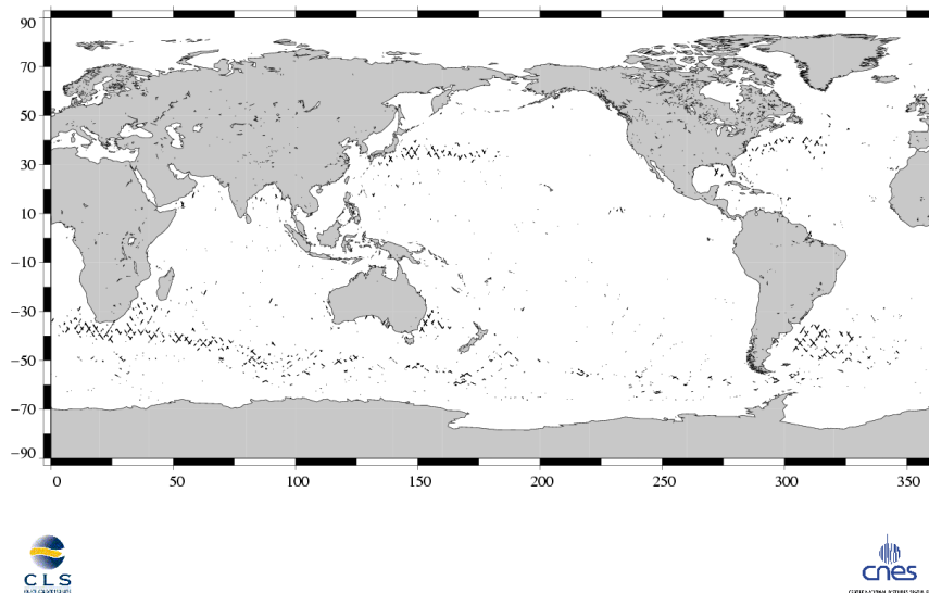
(SSH - MSS) differences greater than 30 cm Jason / Cycle 126
